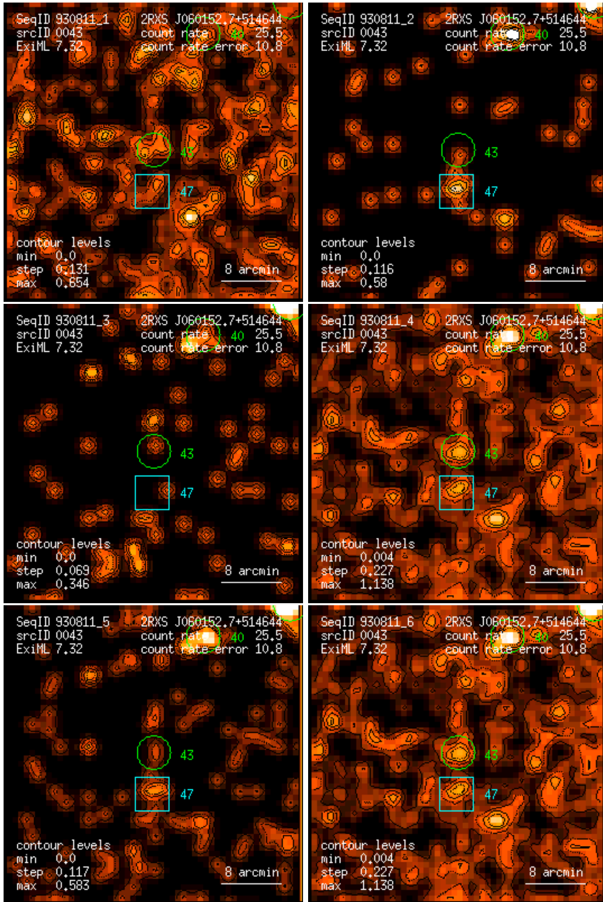
Figure 43: RASS 930811: detection 0043: band rate images, Gaussian filter: (1) PSPC channels 11 – 41, (2) 52 – 90, (3) 91 – 201, (4) 11 – 235, (5) 52 – 201, (6) 11 – 201. Broad band rates in counts/ks. Band rate contour levels in counts/ks/arcmin 2 .
