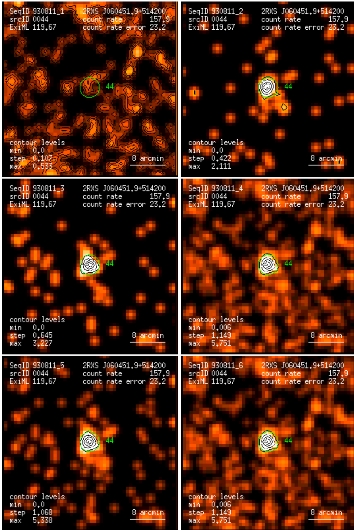
Figure 44: RASS 930811: detection 0044: band rate images, Gaussian filter: (1) PSPC channels 11 – 41, (2) 52 – 90, (3) 91 – 201, (4) 11 – 235, (5) 52 – 201, (6) 11 – 201. Broad band rates in counts/ks. Band rate contour levels in counts/ks/arcmin 2 .
