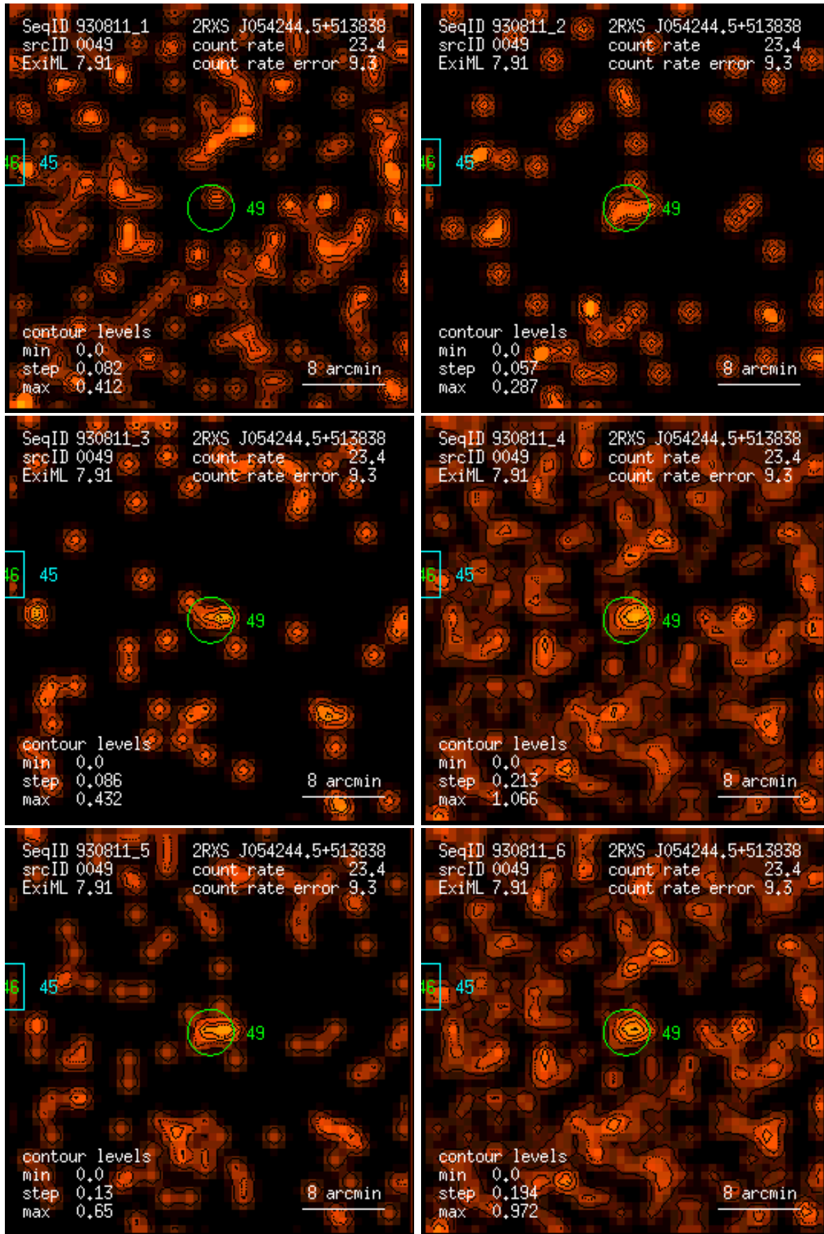
Figure 49: RASS 930811: detection 0049: band rate images, Gaussian filter: (1) PSPC channels 11 – 41, (2) 52 – 90, (3) 91 – 201, (4) 11 – 235, (5) 52 – 201, (6) 11 – 201. Broad band rates in counts/ks. Band rate contour levels in counts/ks/arcmin 2 .
