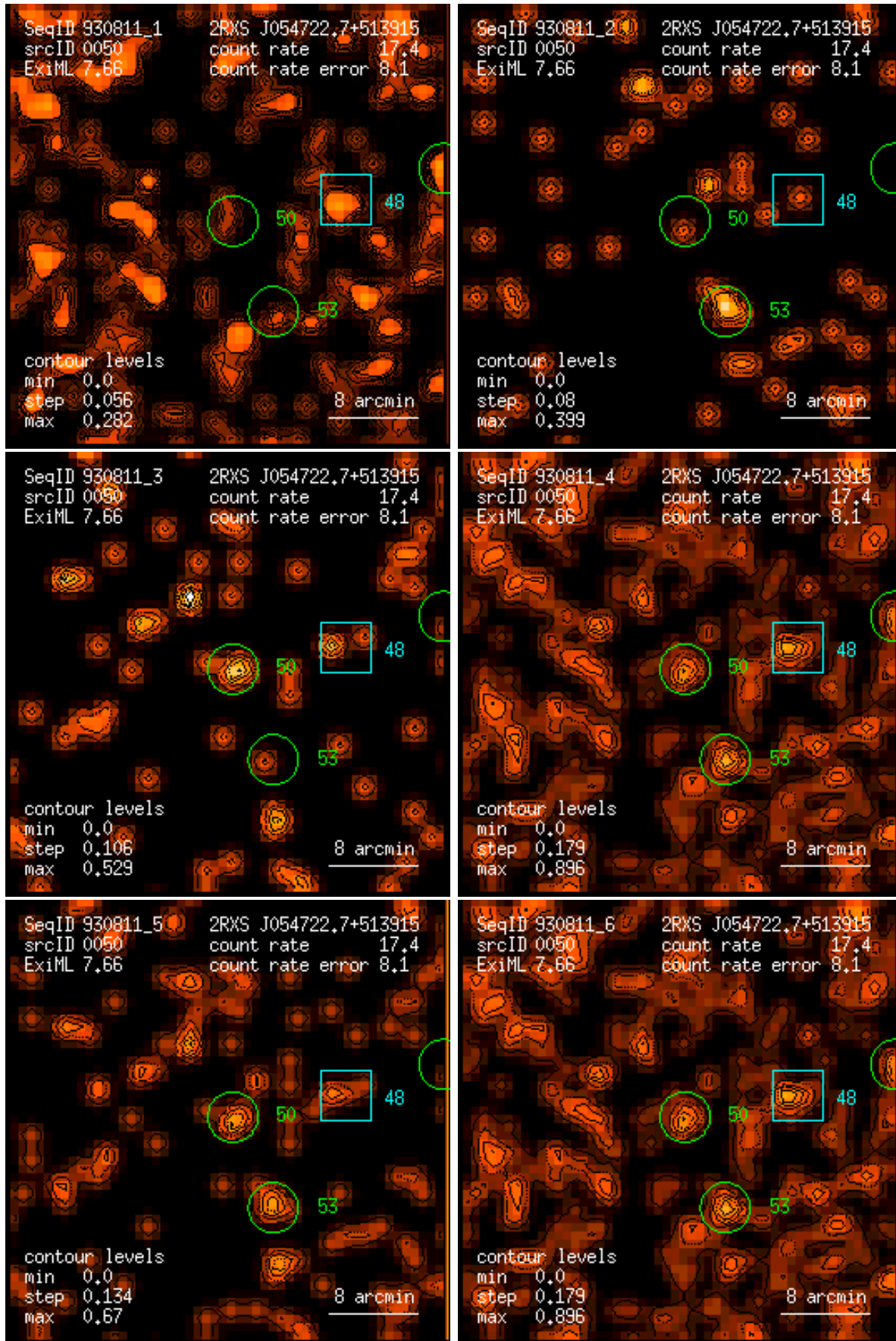
Figure 50: RASS 930811: detection 0050: band rate images, Gaussian filter: (1) PSPC channels 11 – 41, (2) 52 – 90, (3) 91 – 201, (4) 11 – 235, (5) 52 – 201, (6) 11 – 201. Broad band rates in counts/ks. Band rate contour levels in counts/ks/arcmin 2 .
