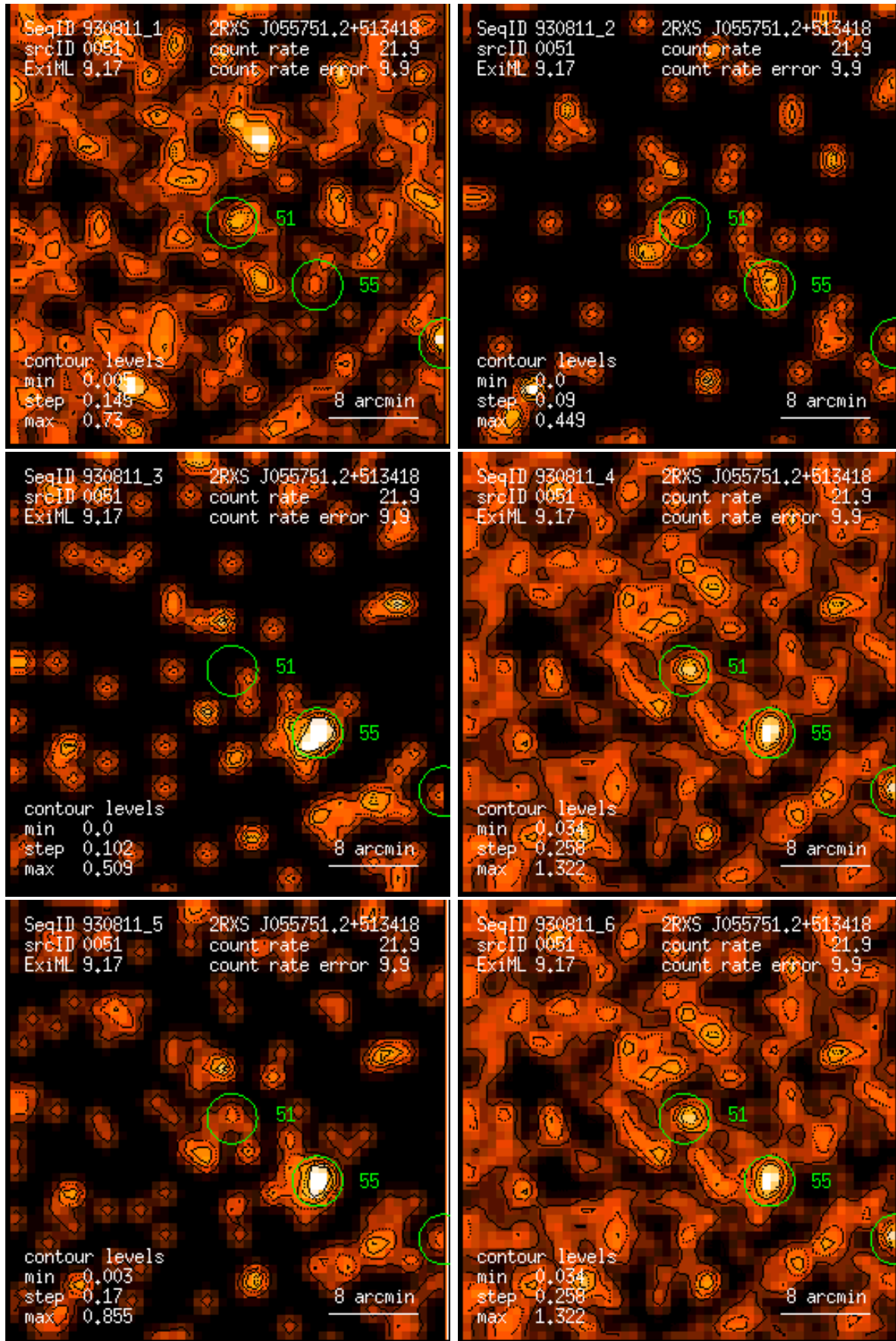
Figure 51: RASS 930811: detection 0051: band rate images, Gaussian filter: (1) PSPC channels 11 – 41, (2) 52 – 90, (3) 91 – 201, (4) 11 – 235, (5) 52 – 201, (6) 11 – 201. Broad band rates in counts/ks. Band rate contour levels in counts/ks/arcmin 2 .
