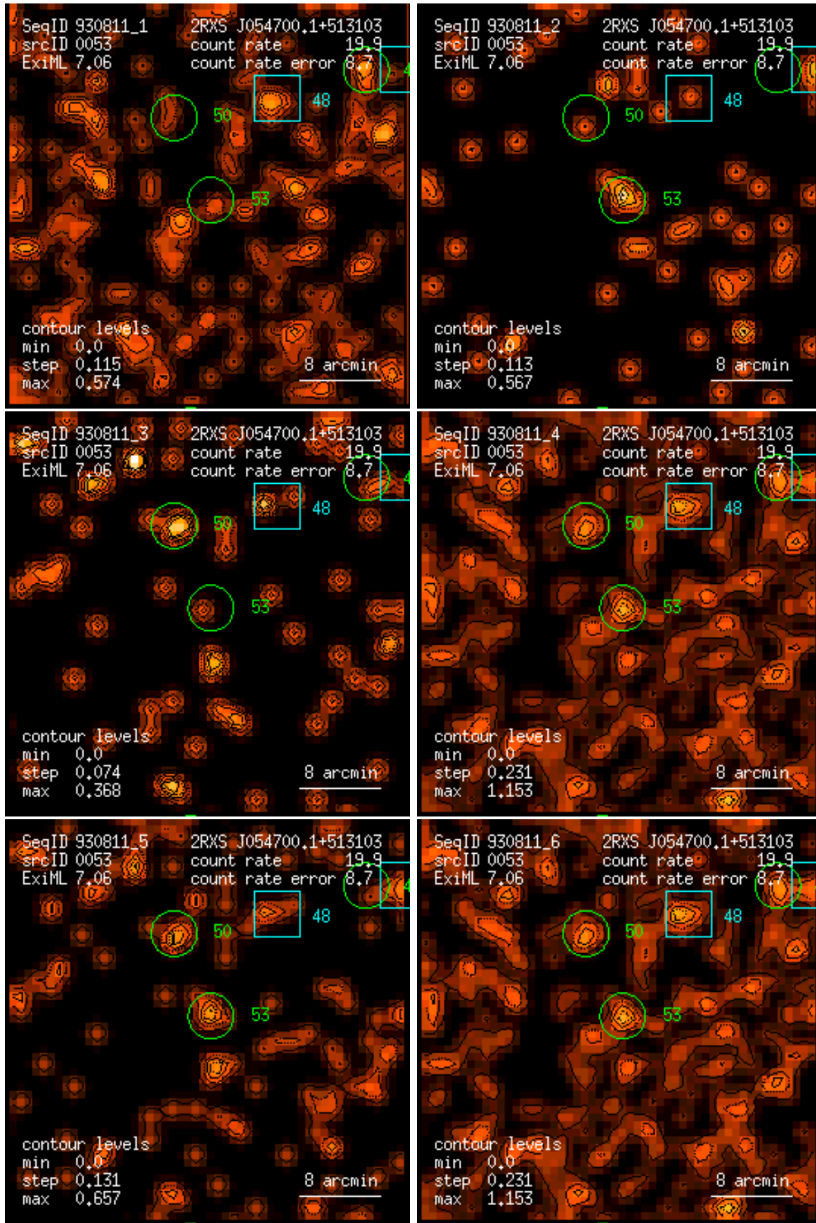
Figure 53: RASS 930811: detection 0053: band rate images, Gaussian filter: (1) PSPC channels 11 – 41, (2) 52 – 90, (3) 91 – 201, (4) 11 – 235, (5) 52 – 201, (6) 11 – 201. Broad band rates in counts/ks. Band rate contour levels in counts/ks/arcmin 2 .
