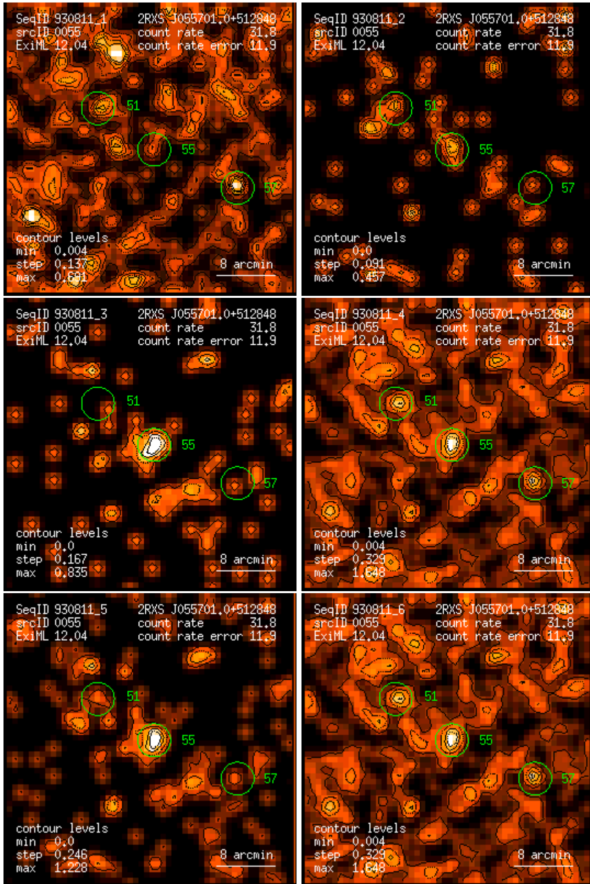
Figure 55: RASS 930811: detection 0055: band rate images, Gaussian filter: (1) PSPC channels 11 – 41, (2) 52 – 90, (3) 91 – 201, (4) 11 – 235, (5) 52 – 201, (6) 11 – 201. Broad band rates in counts/ks. Band rate contour levels in counts/ks/arcmin 2 .
