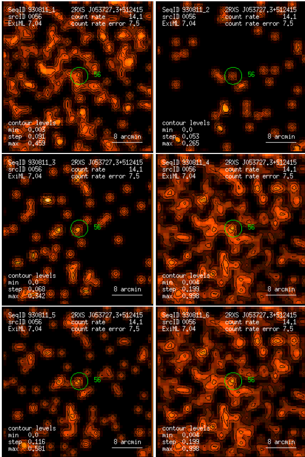
Figure 56: RASS 930811: detection 0056: band rate images, Gaussian filter: (1) PSPC channels 11 – 41, (2) 52 – 90, (3) 91 – 201, (4) 11 – 235, (5) 52 – 201, (6) 11 – 201. Broad band rates in counts/ks. Band rate contour levels in counts/ks/arcmin 2 .
