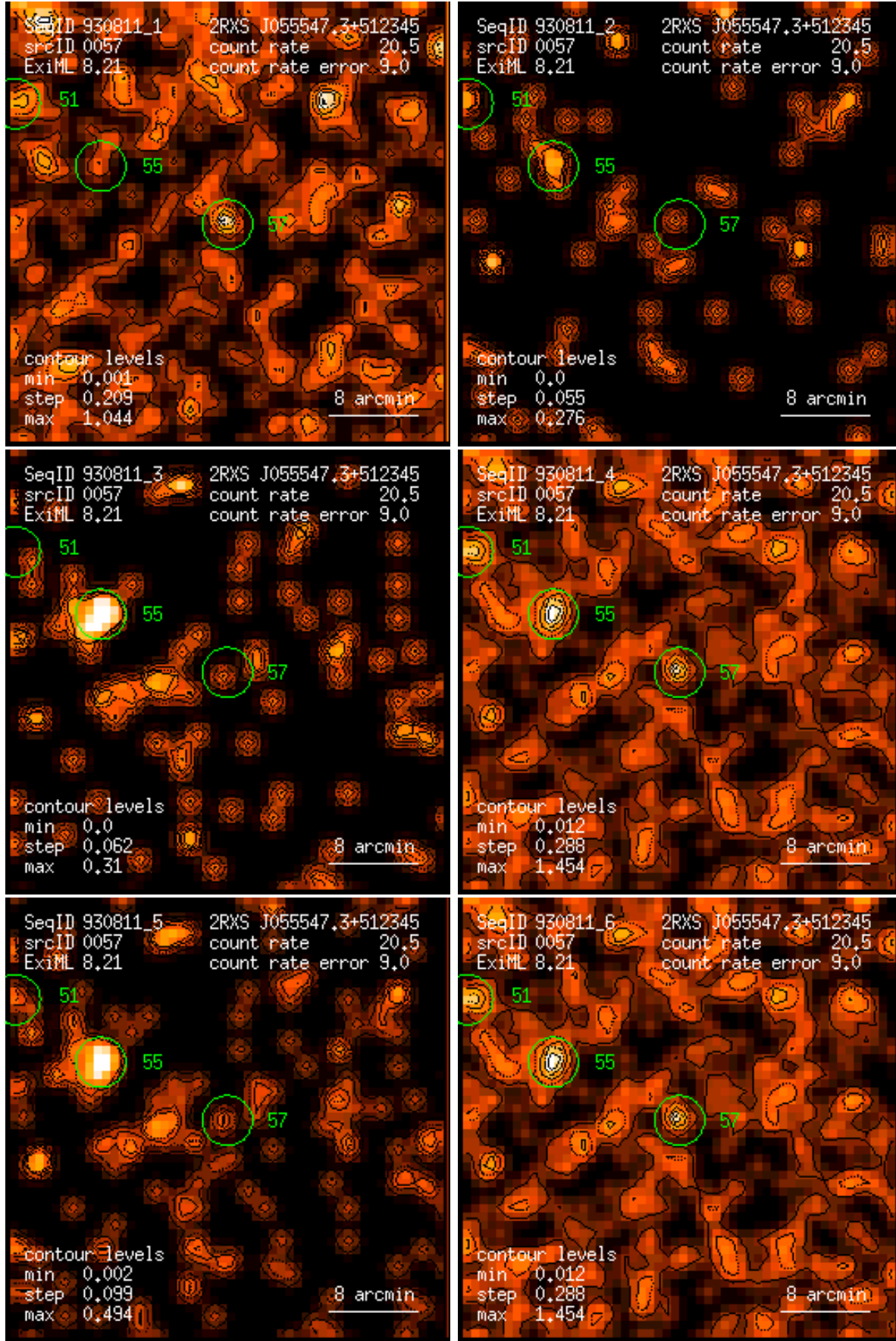
Figure 57: RASS 930811: detection 0057: band rate images, Gaussian filter: (1) PSPC channels 11 – 41, (2) 52 – 90, (3) 91 – 201, (4) 11 – 235, (5) 52 – 201, (6) 11 – 201. Broad band rates in counts/ks. Band rate contour levels in counts/ks/arcmin 2 .
