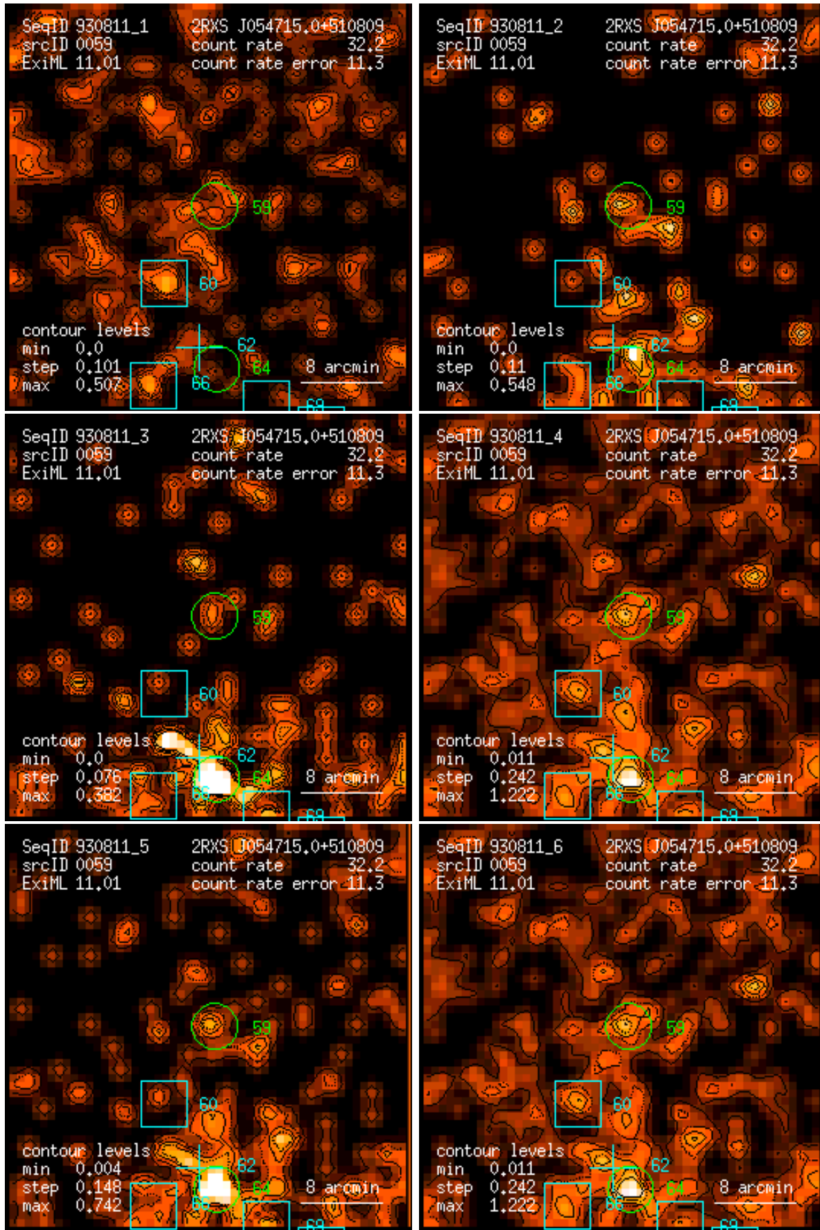
Figure 59: RASS 930811: detection 0059: band rate images, Gaussian filter: (1) PSPC channels 11 – 41, (2) 52 – 90, (3) 91 – 201, (4) 11 – 235, (5) 52 – 201, (6) 11 – 201. Broad band rates in counts/ks. Band rate contour levels in counts/ks/arcmin 2 .
