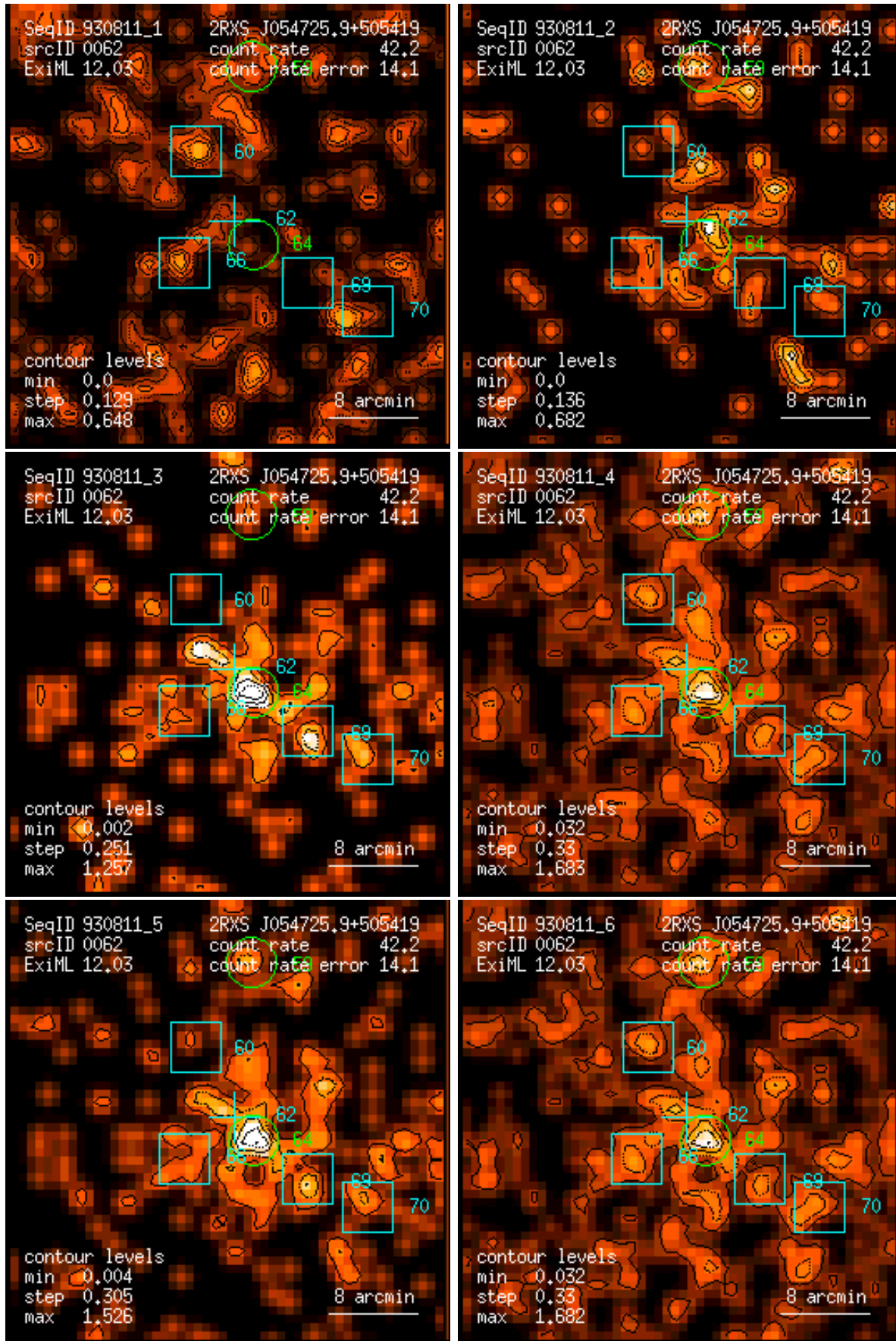
Figure 62: RASS 930811: detection 0062: band rate images, Gaussian filter: (1) PSPC channels 11 – 41, (2) 52 – 90, (3) 91 – 201, (4) 11 – 235, (5) 52 – 201, (6) 11 – 201. Broad band rates in counts/ks. Band rate contour levels in counts/ks/arcmin 2 .
