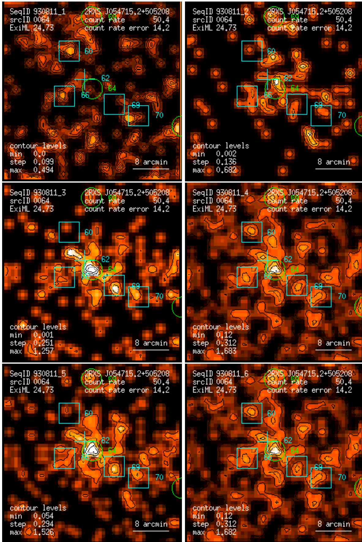
Figure 64: RASS 930811: detection 0064: band rate images, Gaussian filter: (1) PSPC channels 11 – 41, (2) 52 – 90, (3) 91 – 201, (4) 11 – 235, (5) 52 – 201, (6) 11 – 201. Broad band rates in counts/ks. Band rate contour levels in counts/ks/arcmin 2 .
