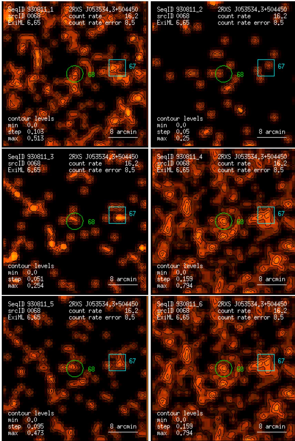
Figure 68: RASS 930811: detection 0068: band rate images, Gaussian filter: (1) PSPC channels 11 – 41, (2) 52 – 90, (3) 91 – 201, (4) 11 – 235, (5) 52 – 201, (6) 11 – 201. Broad band rates in counts/ks. Band rate contour levels in counts/ks/arcmin 2 .
