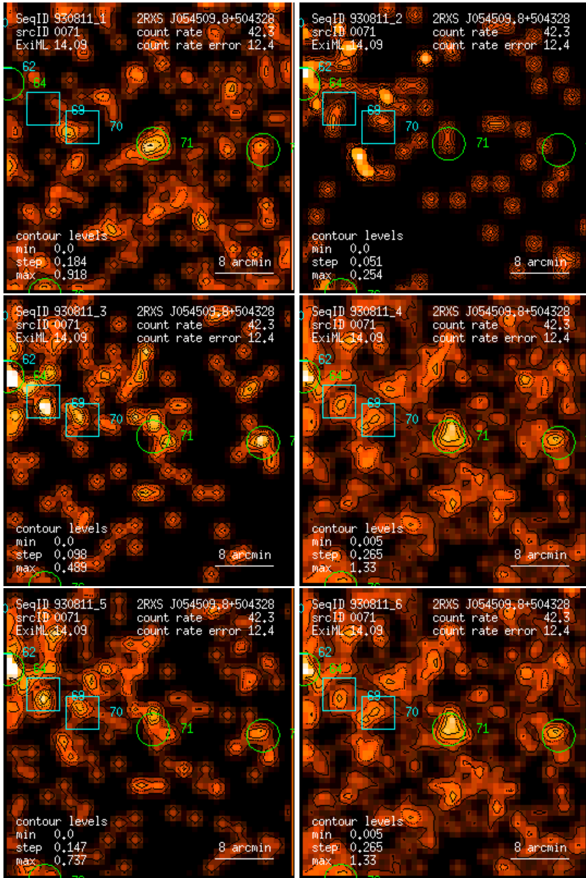
Figure 71: RASS 930811: detection 0071: band rate images, Gaussian filter: (1) PSPC channels 11 – 41, (2) 52 – 90, (3) 91 – 201, (4) 11 – 235, (5) 52 – 201, (6) 11 – 201. Broad band rates in counts/ks. Band rate contour levels in counts/ks/arcmin 2 .
