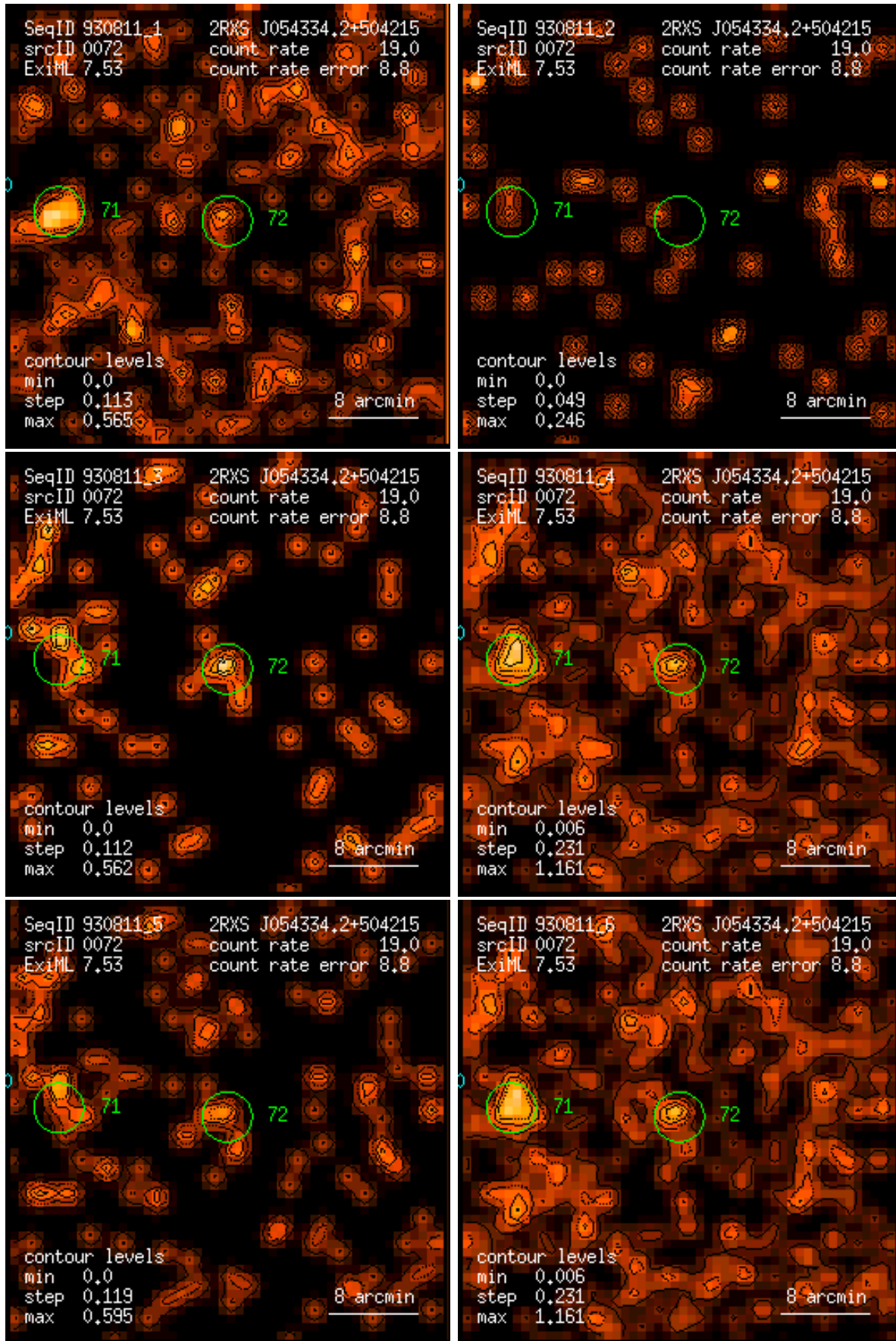
Figure 72: RASS 930811: detection 0072: band rate images, Gaussian filter: (1) PSPC channels 11 – 41, (2) 52 – 90, (3) 91 – 201, (4) 11 – 235, (5) 52 – 201, (6) 11 – 201. Broad band rates in counts/ks. Band rate contour levels in counts/ks/arcmin 2 .
