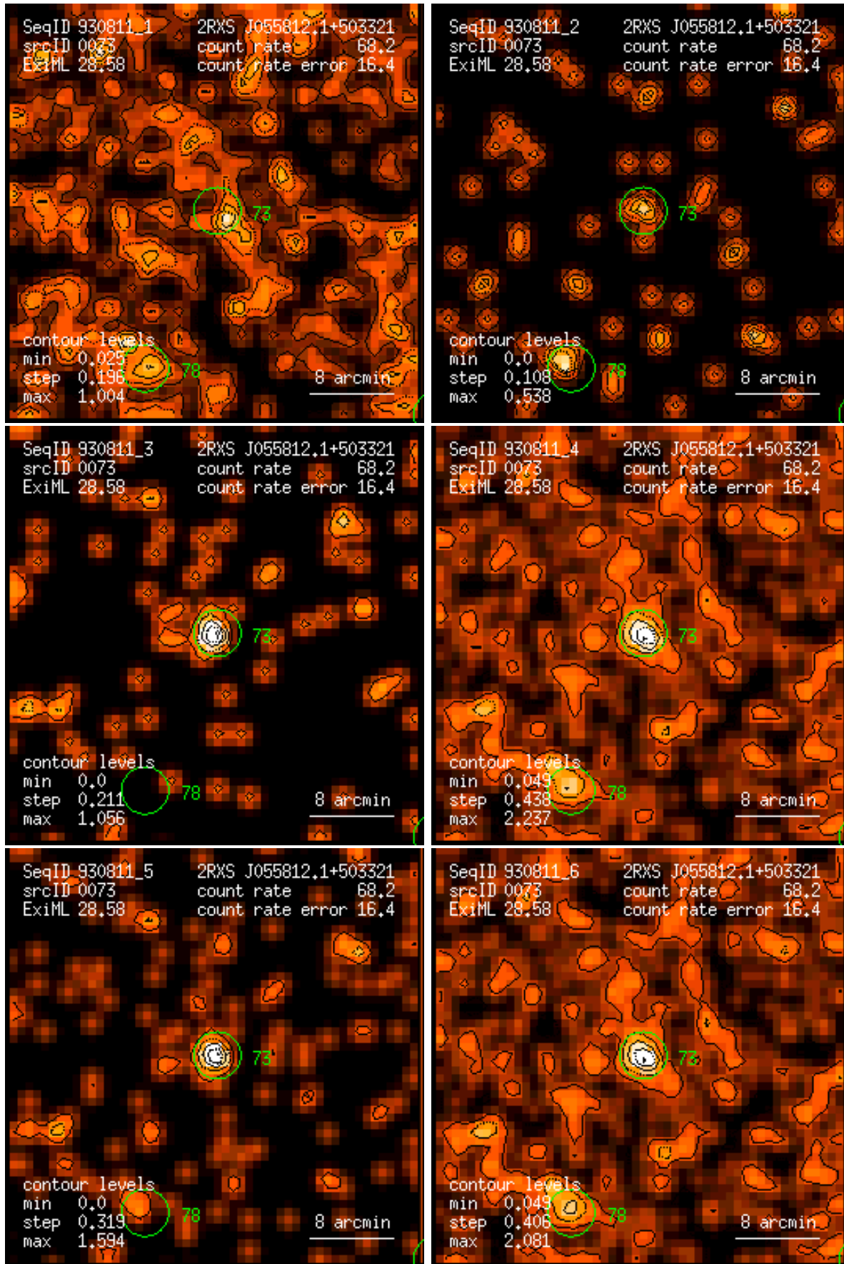
Figure 73: RASS 930811: detection 0073: band rate images, Gaussian filter: (1) PSPC channels 11 – 41, (2) 52 – 90, (3) 91 – 201, (4) 11 – 235, (5) 52 – 201, (6) 11 – 201. Broad band rates in counts/ks. Band rate contour levels in counts/ks/arcmin 2 .
