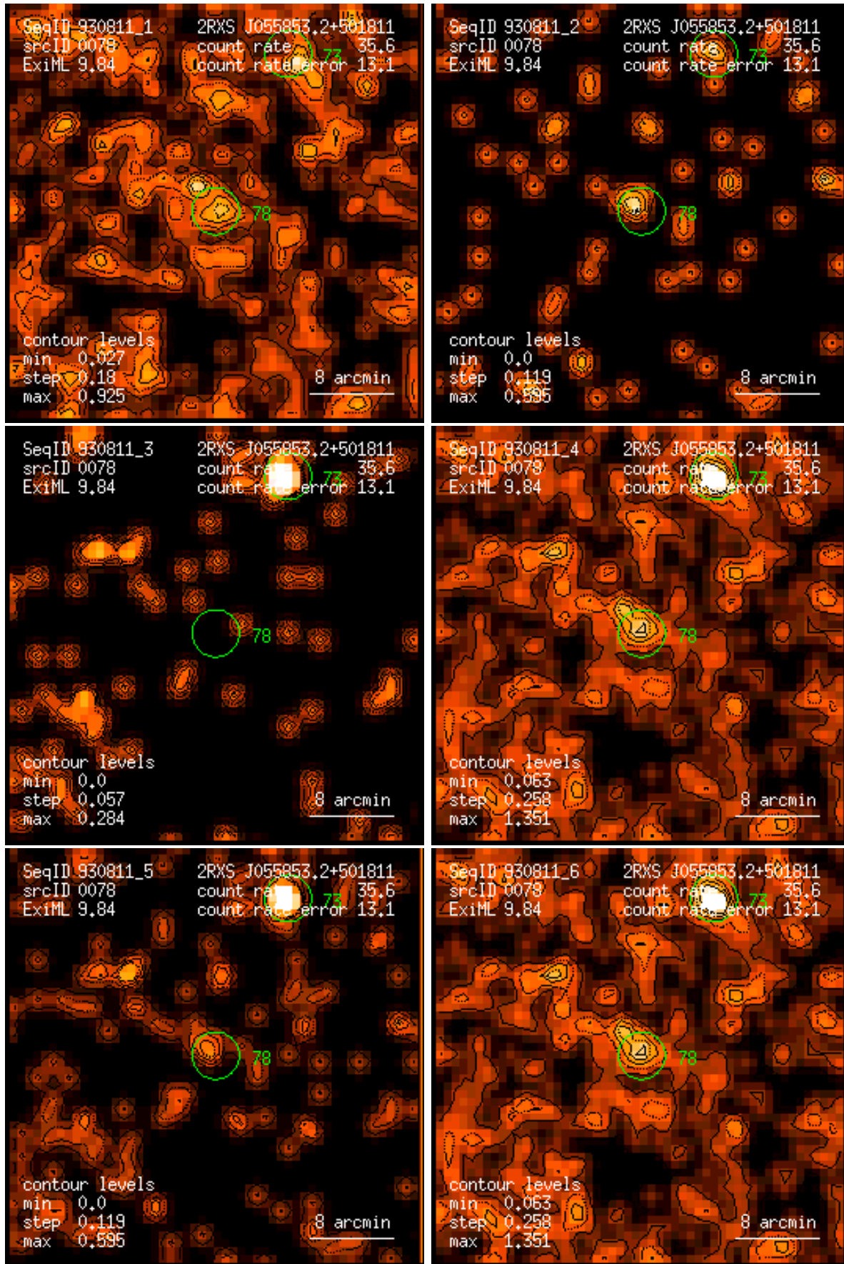
Figure 78: RASS 930811: detection 0078: band rate images, Gaussian filter: (1) PSPC channels 11 – 41, (2) 52 – 90, (3) 91 – 201, (4) 11 – 235, (5) 52 – 201, (6) 11 – 201. Broad band rates in counts/ks. Band rate contour levels in counts/ks/arcmin 2 .
