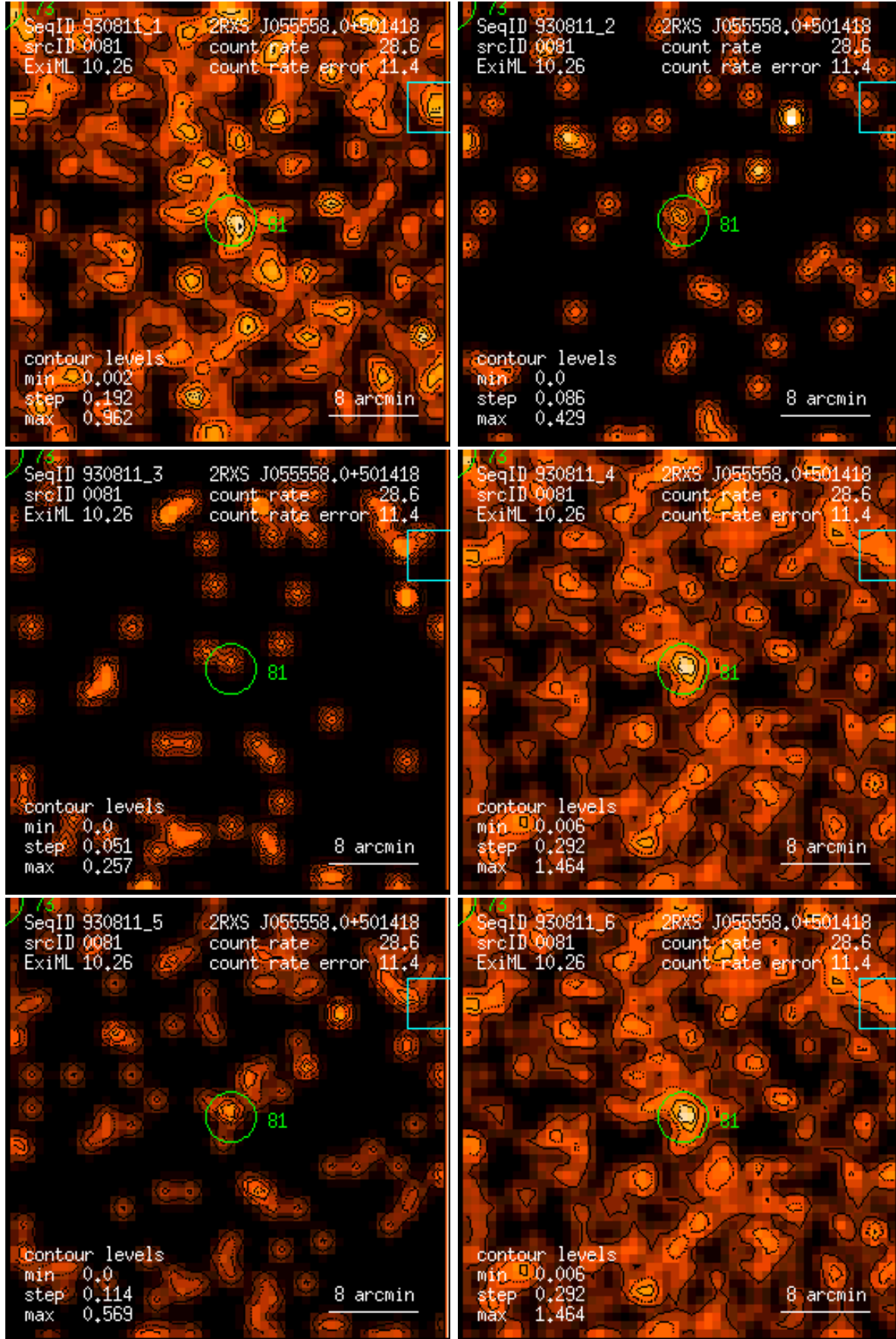
Figure 81: RASS 930811: detection 0081: band rate images, Gaussian filter: (1) PSPC channels 11 – 41, (2) 52 – 90, (3) 91 – 201, (4) 11 – 235, (5) 52 – 201, (6) 11 – 201. Broad band rates in counts/ks. Band rate contour levels in counts/ks/arcmin 2 .
