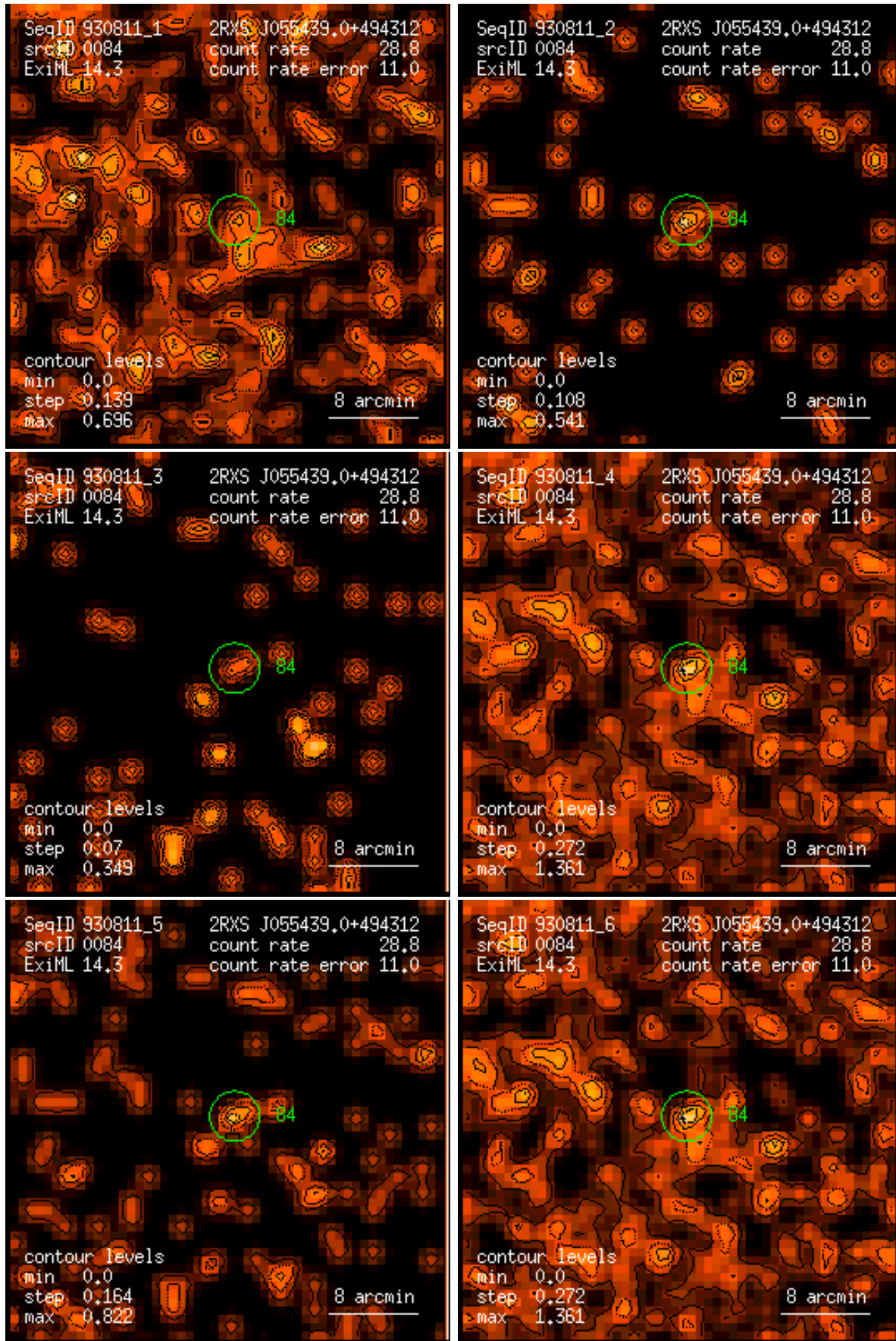
Figure 84: RASS 930811: detection 0084: band rate images, Gaussian filter: (1) PSPC channels 11 – 41, (2) 52 – 90, (3) 91 – 201, (4) 11 – 235, (5) 52 – 201, (6) 11 – 201. Broad band rates in counts/ks. Band rate contour levels in counts/ks/arcmin 2 .
