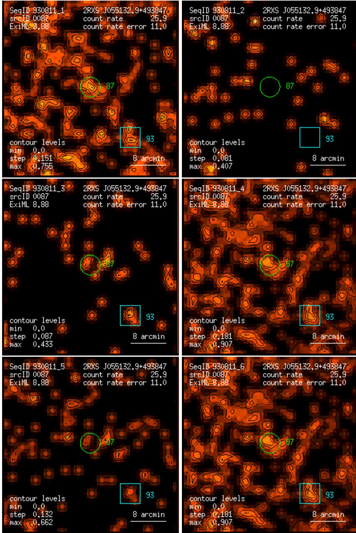
Figure 87: RASS 930811: detection 0087: band rate images, Gaussian filter: (1) PSPC channels 11 – 41, (2) 52 – 90, (3) 91 – 201, (4) 11 – 235, (5) 52 – 201, (6) 11 – 201. Broad band rates in counts/ks. Band rate contour levels in counts/ks/arcmin 2 .
