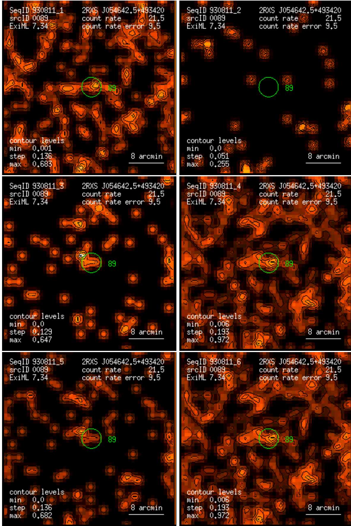
Figure 89: RASS 930811: detection 0089: band rate images, Gaussian filter: (1) PSPC channels 11 – 41, (2) 52 – 90, (3) 91 – 201, (4) 11 – 235, (5) 52 – 201, (6) 11 – 201. Broad band rates in counts/ks. Band rate contour levels in counts/ks/arcmin 2 .
