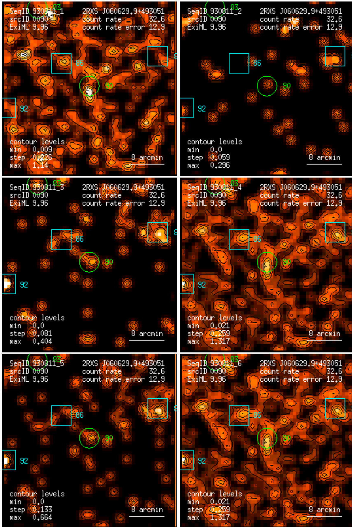
Figure 90: RASS 930811: detection 0090: band rate images, Gaussian filter: (1) PSPC channels 11 – 41, (2) 52 – 90, (3) 91 – 201, (4) 11 – 235, (5) 52 – 201, (6) 11 – 201. Broad band rates in counts/ks. Band rate contour levels in counts/ks/arcmin 2 .
