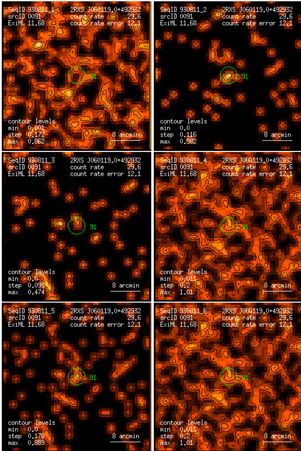
Figure 91: RASS 930811: detection 0091: band rate images, Gaussian filter: (1) PSPC channels 11 – 41, (2) 52 – 90, (3) 91 – 201, (4) 11 – 235, (5) 52 – 201, (6) 11 – 201. Broad band rates in counts/ks. Band rate contour levels in counts/ks/arcmin 2 .
