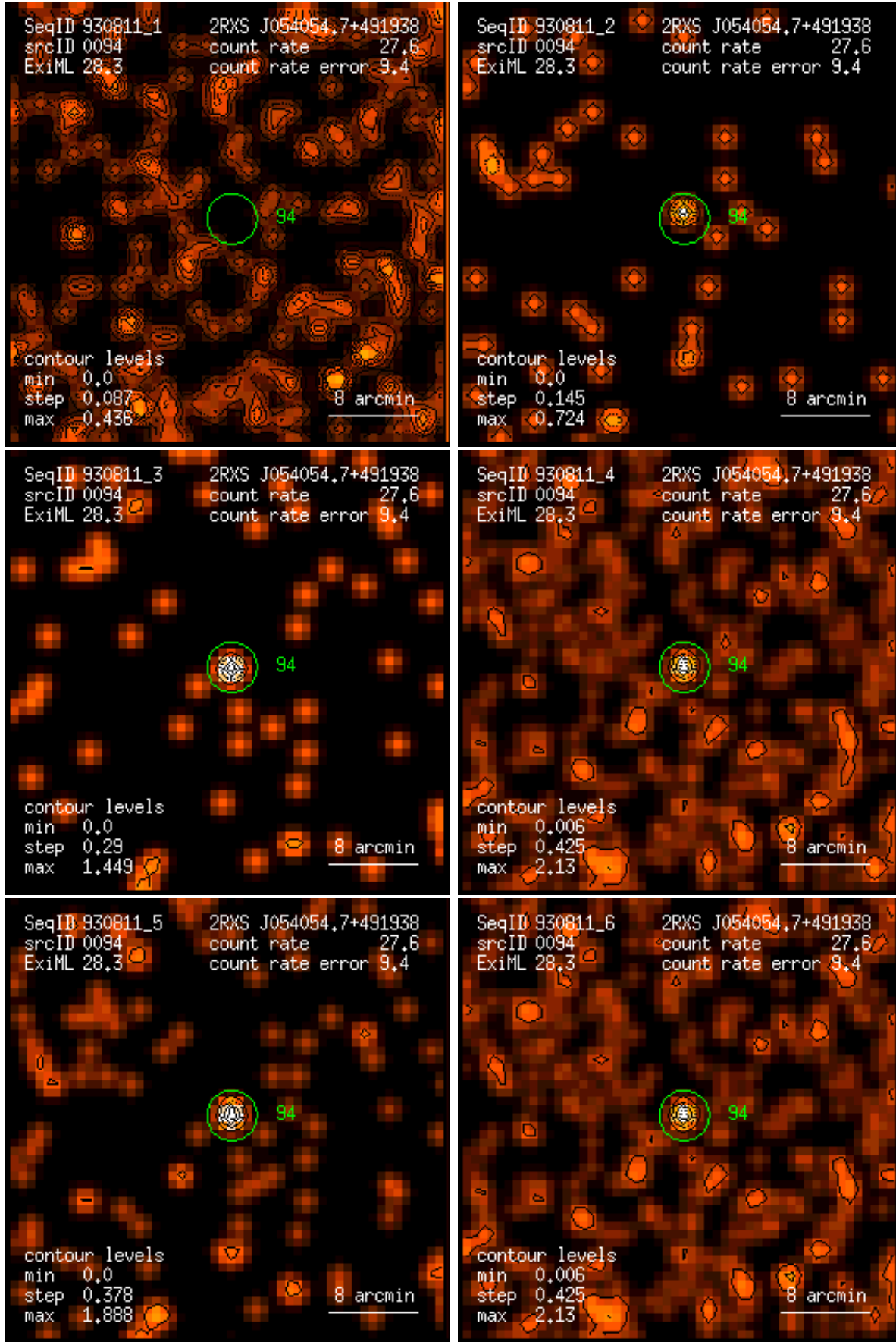
Figure 94: RASS 930811: detection 0094: band rate images, Gaussian filter: (1) PSPC channels 11 – 41, (2) 52 – 90, (3) 91 – 201, (4) 11 – 235, (5) 52 – 201, (6) 11 – 201. Broad band rates in counts/ks. Band rate contour levels in counts/ks/arcmin 2 .
