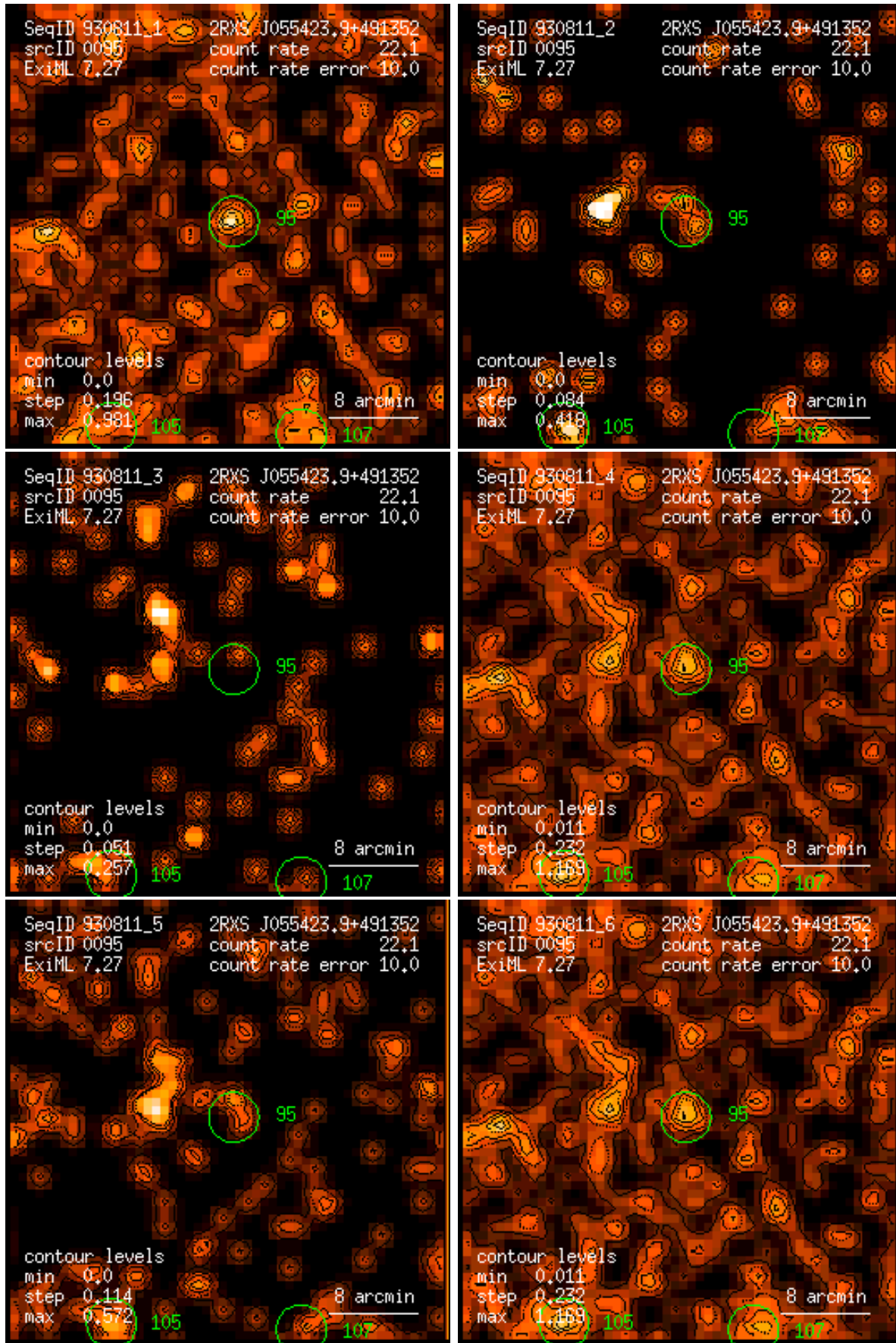
Figure 95: RASS 930811: detection 0095: band rate images, Gaussian filter: (1) PSPC channels 11 – 41, (2) 52 – 90, (3) 91 – 201, (4) 11 – 235, (5) 52 – 201, (6) 11 – 201. Broad band rates in counts/ks. Band rate contour levels in counts/ks/arcmin 2 .
