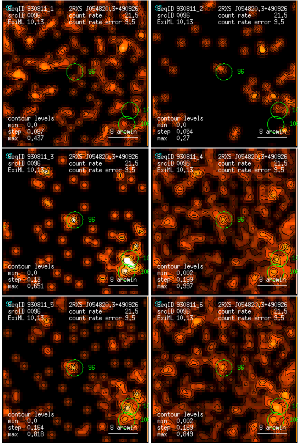
Figure 96: RASS 930811: detection 0096: band rate images, Gaussian filter: (1) PSPC channels 11 – 41, (2) 52 – 90, (3) 91 – 201, (4) 11 – 235, (5) 52 – 201, (6) 11 – 201. Broad band rates in counts/ks. Band rate contour levels in counts/ks/arcmin 2 .
