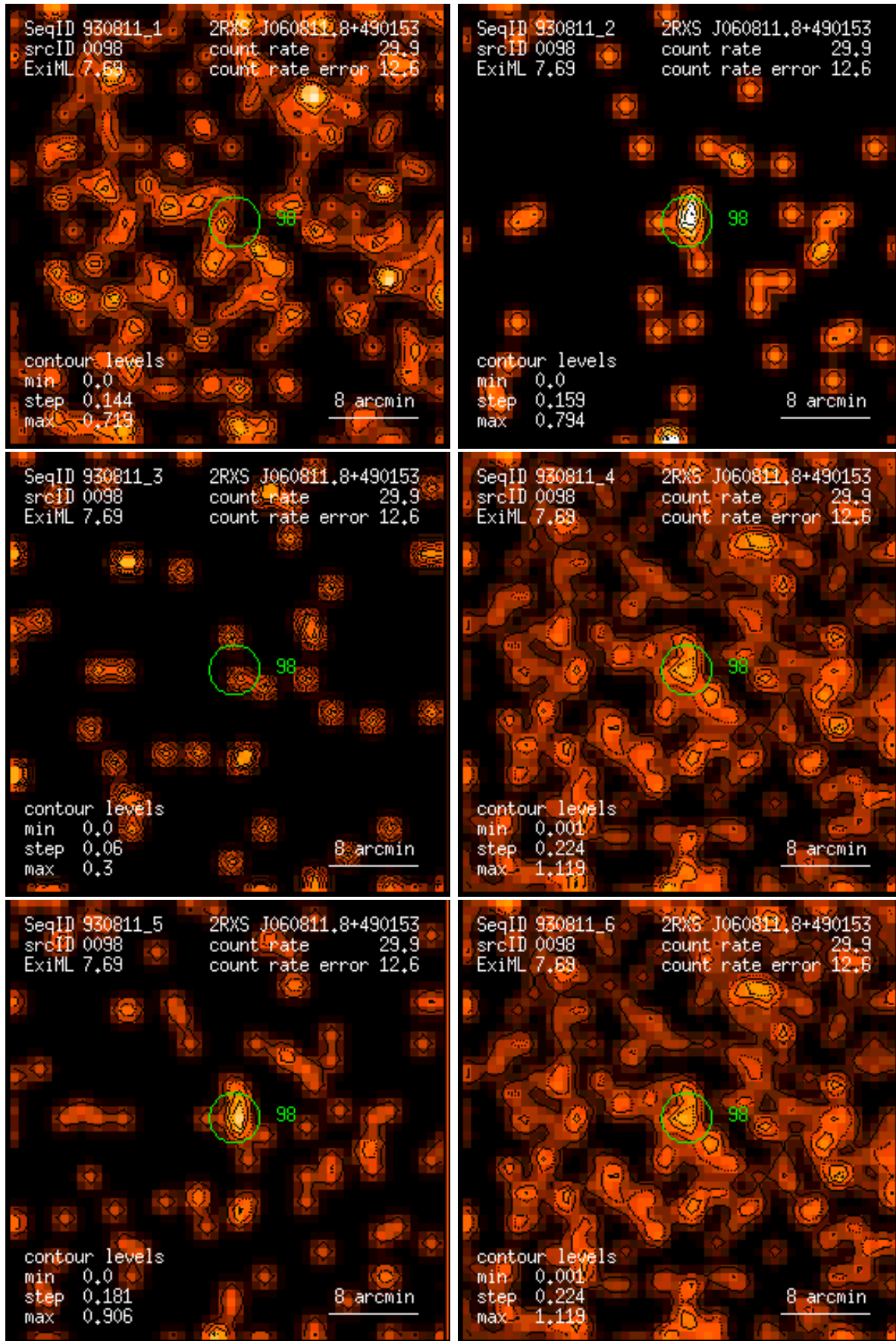
Figure 98: RASS 930811: detection 0098: band rate images, Gaussian filter: (1) PSPC channels 11 – 41, (2) 52 – 90, (3) 91 – 201, (4) 11 – 235, (5) 52 – 201, (6) 11 – 201. Broad band rates in counts/ks. Band rate contour levels in counts/ks/arcmin 2 .
