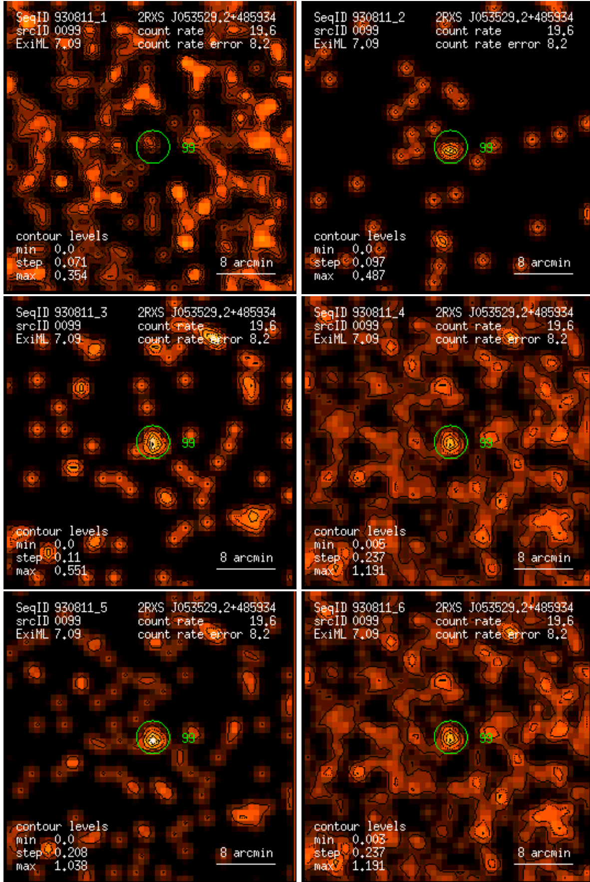
Figure 99: RASS 930811: detection 0099: band rate images, Gaussian filter: (1) PSPC channels 11 – 41, (2) 52 – 90, (3) 91 – 201, (4) 11 – 235, (5) 52 – 201, (6) 11 – 201. Broad band rates in counts/ks. Band rate contour levels in counts/ks/arcmin 2 .
