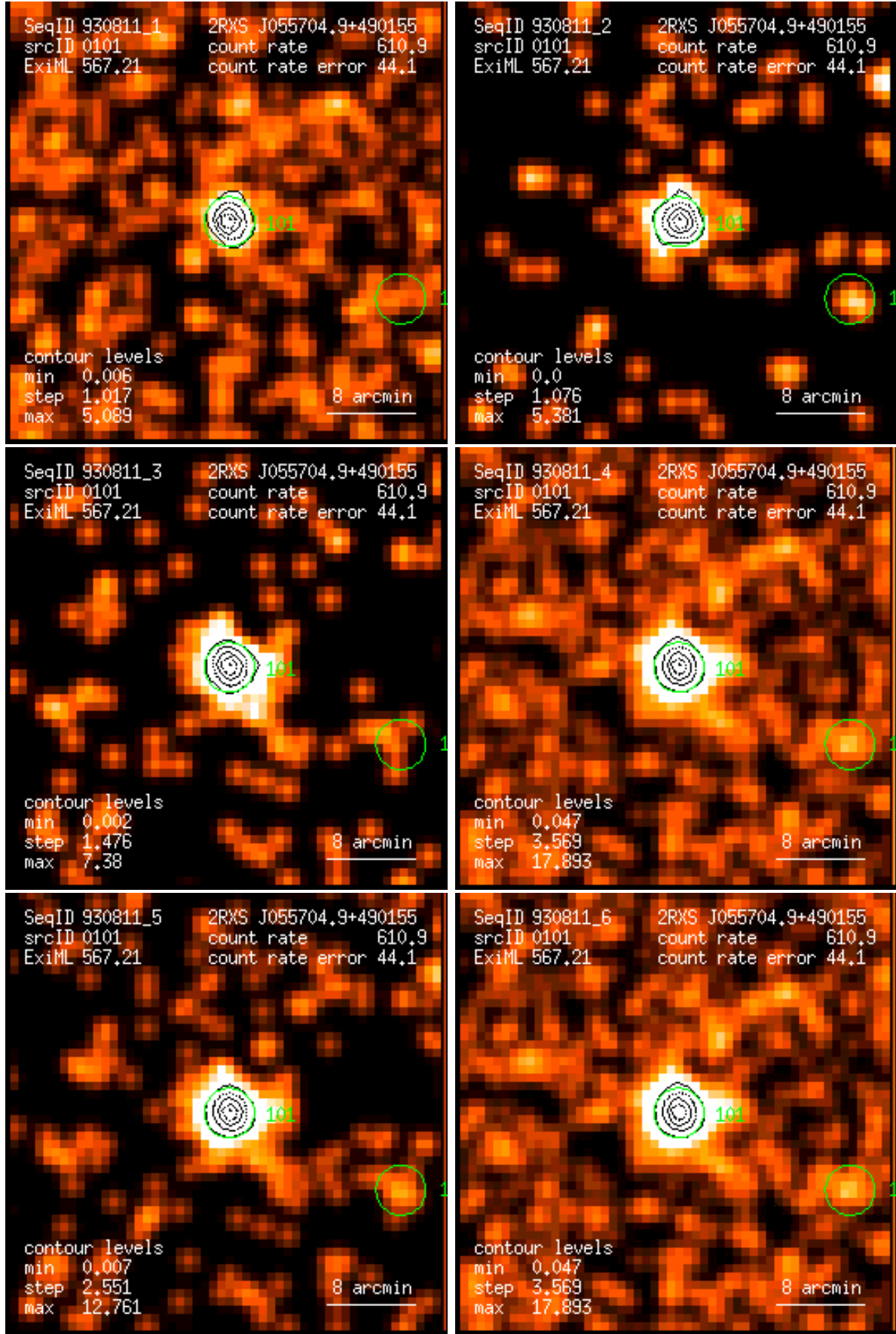
Figure 101: RASS 930811: detection 0101: band rate images, Gaussian filter: (1) PSPC channels 11 – 41, (2) 52 – 90, (3) 91 – 201, (4) 11 – 235, (5) 52 – 201, (6) 11 – 201. Broad band rates in counts/ks. Band rate contour levels in counts/ks/arcmin 2 .
