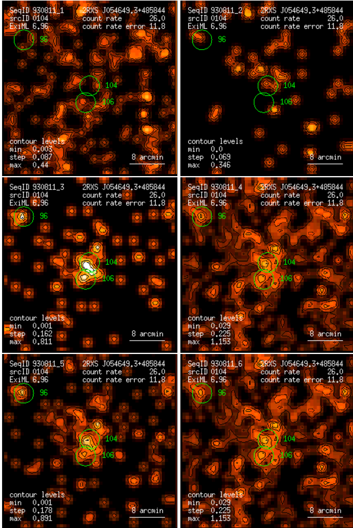
Figure 104: RASS 930811: detection 0104: band rate images, Gaussian filter: (1) PSPC channels 11 – 41, (2) 52 – 90, (3) 91 – 201, (4) 11 – 235, (5) 52 – 201, (6) 11 – 201. Broad band rates in counts/ks. Band rate contour levels in counts/ks/arcmin 2 .
