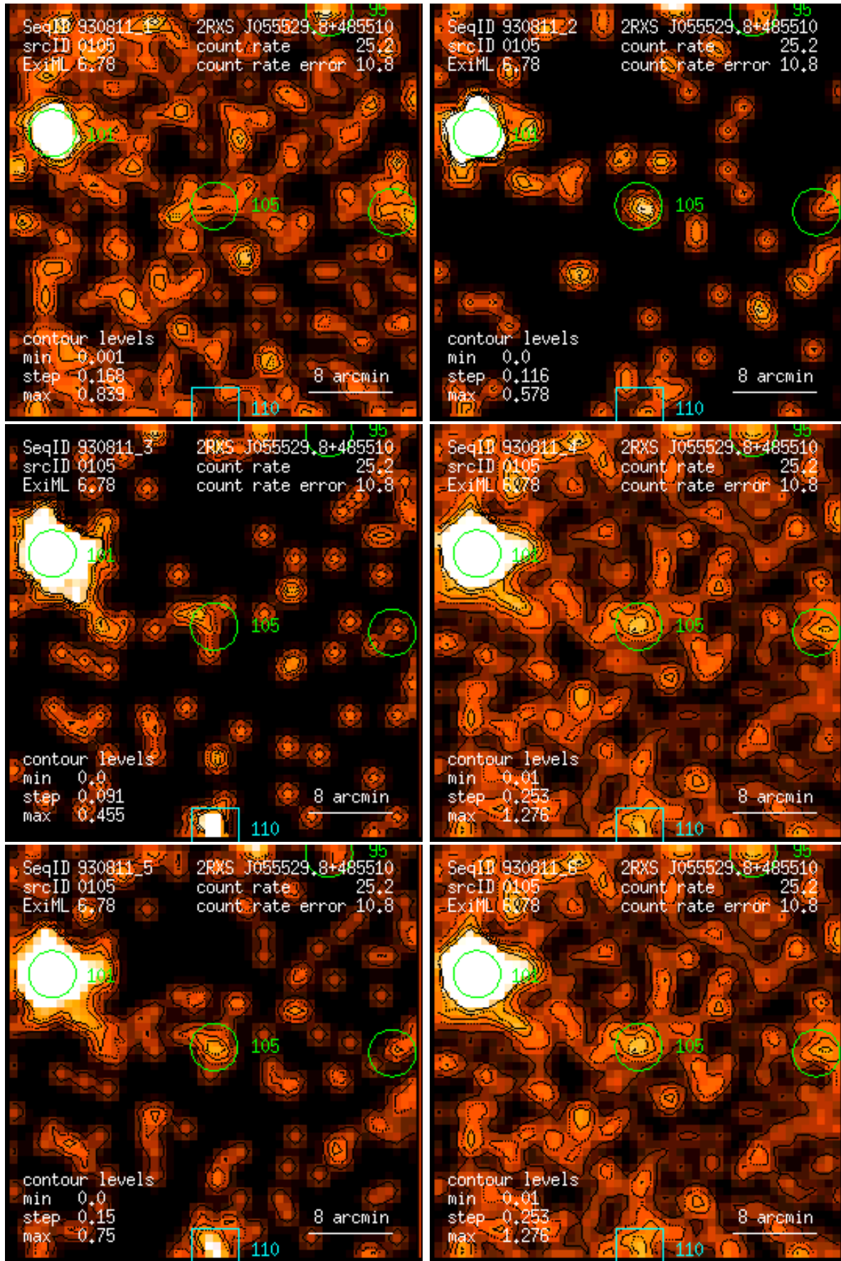
Figure 105: RASS 930811: detection 0105: band rate images, Gaussian filter: (1) PSPC channels 11 – 41, (2) 52 – 90, (3) 91 – 201, (4) 11 – 235, (5) 52 – 201, (6) 11 – 201. Broad band rates in counts/ks. Band rate contour levels in counts/ks/arcmin 2 .
