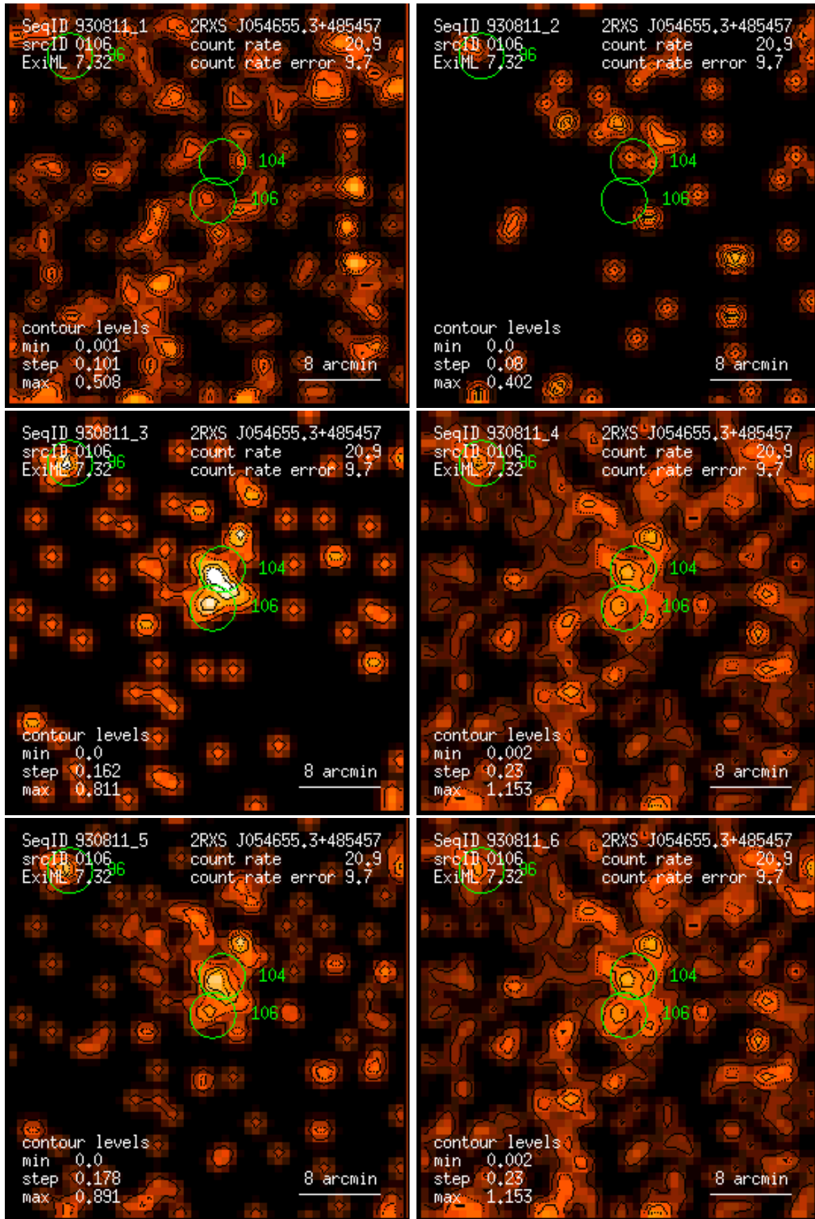
Figure 106: RASS 930811: detection 0106: band rate images, Gaussian filter: (1) PSPC channels 11 – 41, (2) 52 – 90, (3) 91 – 201, (4) 11 – 235, (5) 52 – 201, (6) 11 – 201. Broad band rates in counts/ks. Band rate contour levels in counts/ks/arcmin 2 .
