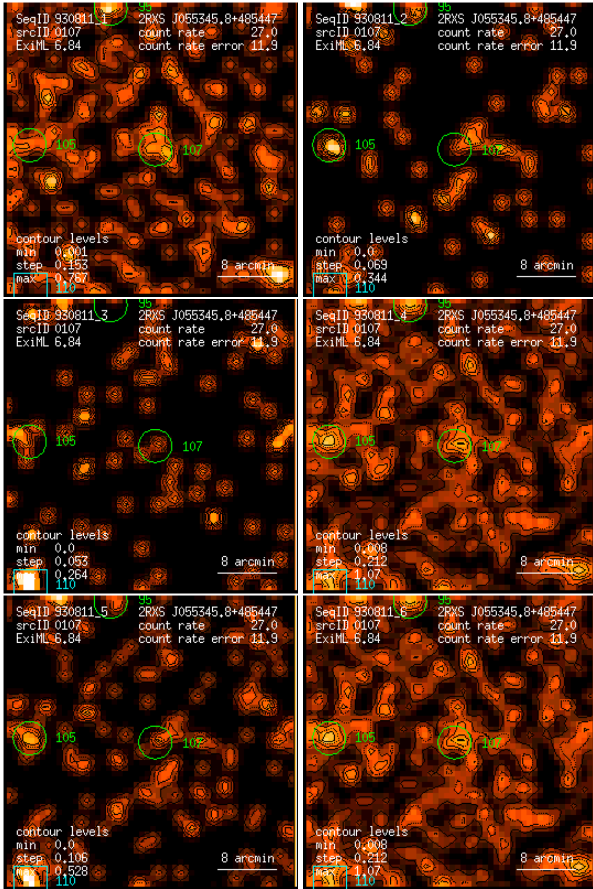
Figure 107: RASS 930811: detection 0107: band rate images, Gaussian filter: (1) PSPC channels 11 – 41, (2) 52 – 90, (3) 91 – 201, (4) 11 – 235, (5) 52 – 201, (6) 11 – 201. Broad band rates in counts/ks. Band rate contour levels in counts/ks/arcmin 2 .
