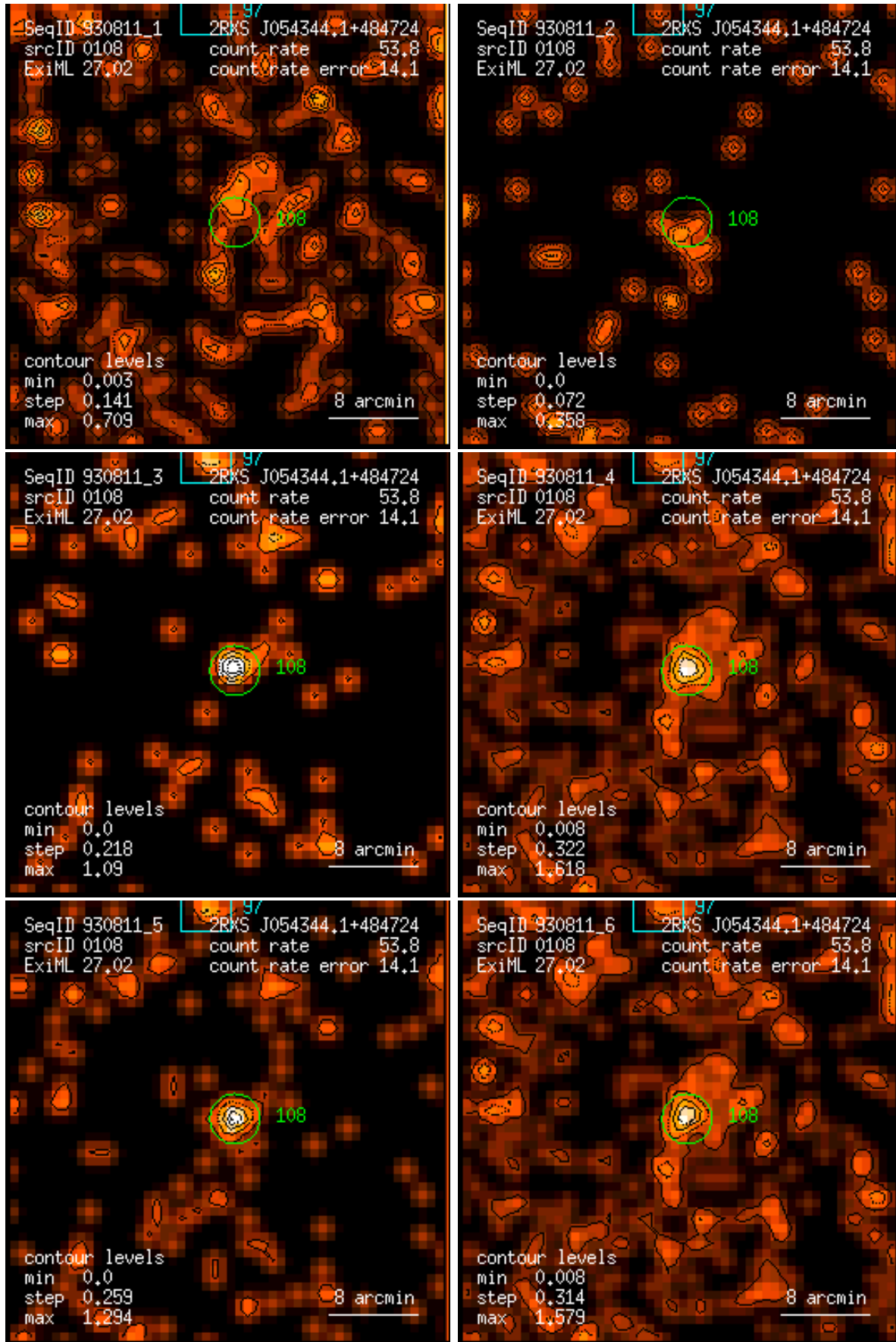
Figure 108: RASS 930811: detection 0108: band rate images, Gaussian filter: (1) PSPC channels 11 – 41, (2) 52 – 90, (3) 91 – 201, (4) 11 – 235, (5) 52 – 201, (6) 11 – 201. Broad band rates in counts/ks. Band rate contour levels in counts/ks/arcmin 2 .
