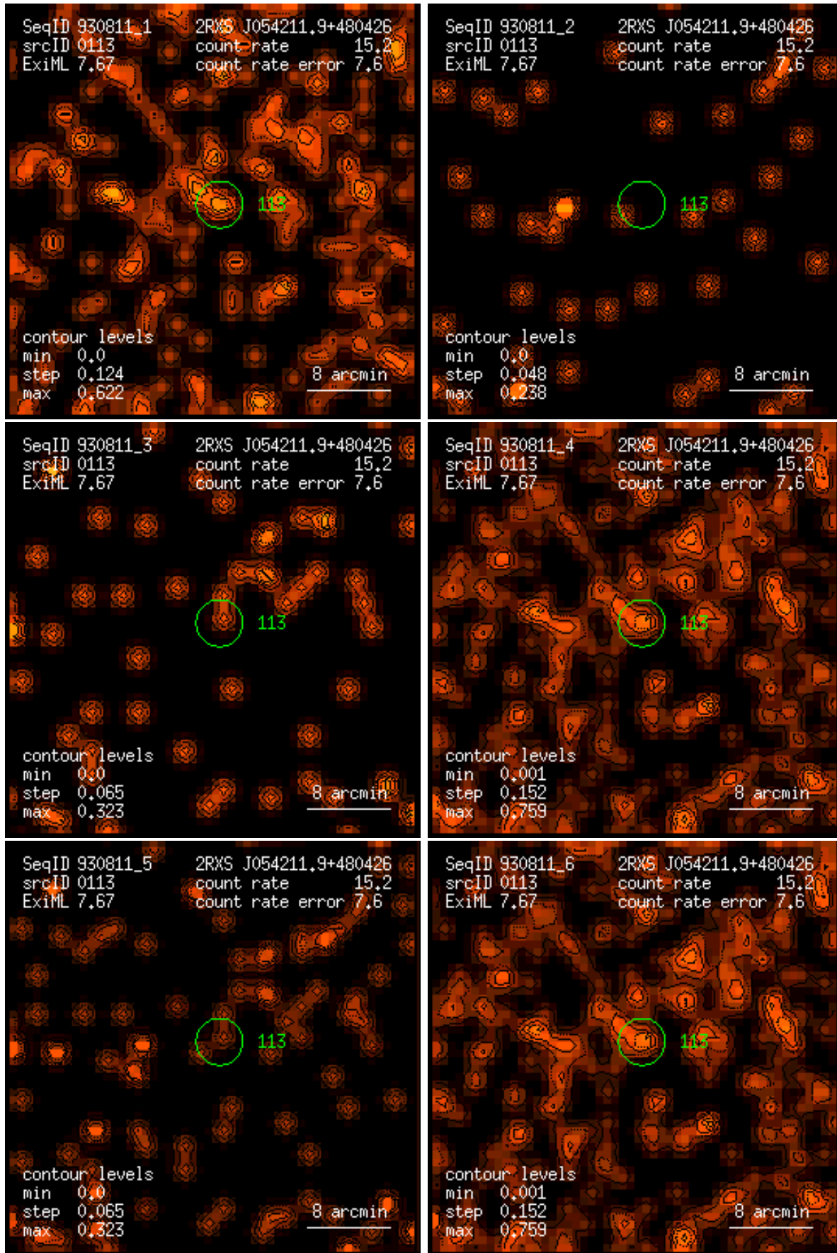
Figure 113: RASS 930811: detection 0113: band rate images, Gaussian filter: (1) PSPC channels 11 – 41, (2) 52 – 90, (3) 91 – 201, (4) 11 – 235, (5) 52 – 201, (6) 11 – 201. Broad band rates in counts/ks. Band rate contour levels in counts/ks/arcmin 2 .
