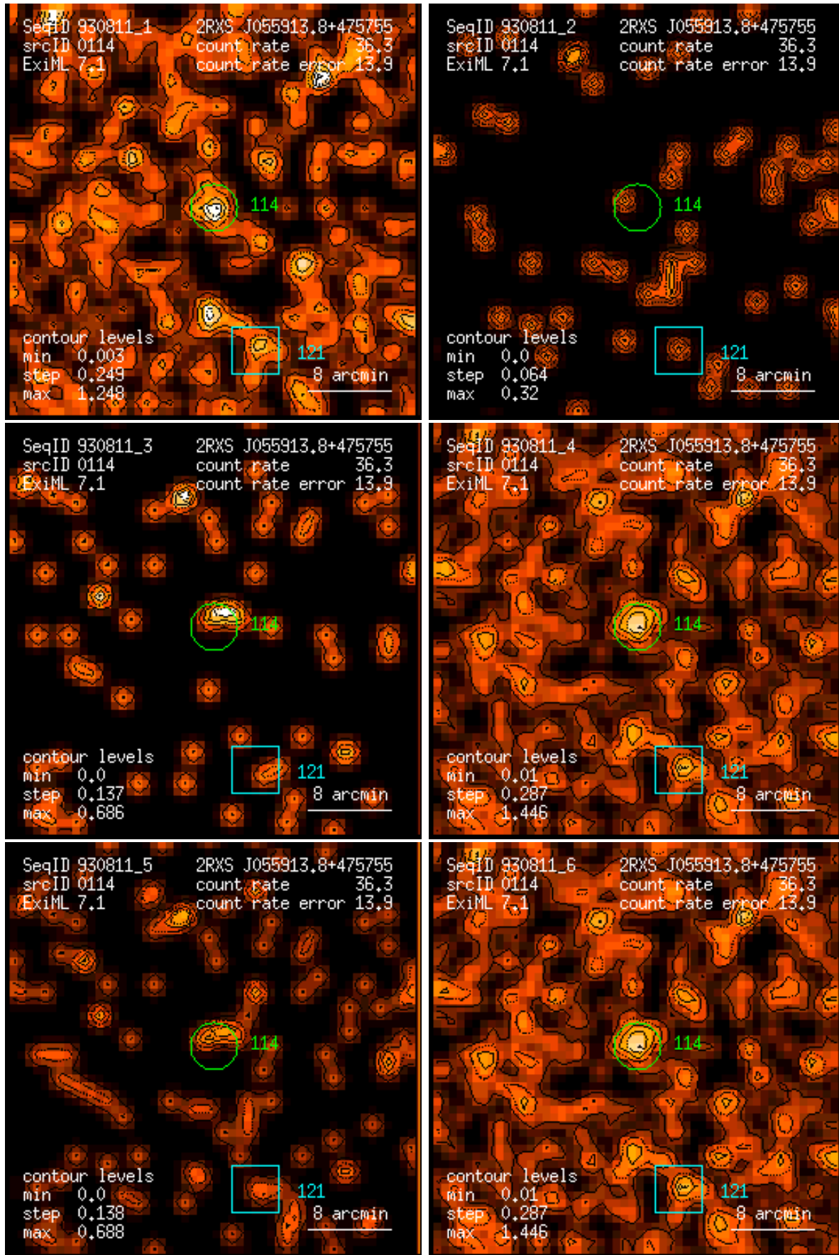
Figure 114: RASS 930811: detection 0114: band rate images, Gaussian filter: (1) PSPC channels 11 – 41, (2) 52 – 90, (3) 91 – 201, (4) 11 – 235, (5) 52 – 201, (6) 11 – 201. Broad band rates in counts/ks. Band rate contour levels in counts/ks/arcmin 2 .
