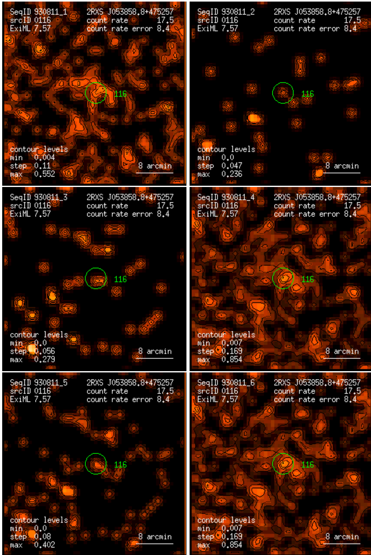
Figure 116: RASS 930811: detection 0116: band rate images, Gaussian filter: (1) PSPC channels 11 – 41, (2) 52 – 90, (3) 91 – 201, (4) 11 – 235, (5) 52 – 201, (6) 11 – 201. Broad band rates in counts/ks. Band rate contour levels in counts/ks/arcmin 2 .
