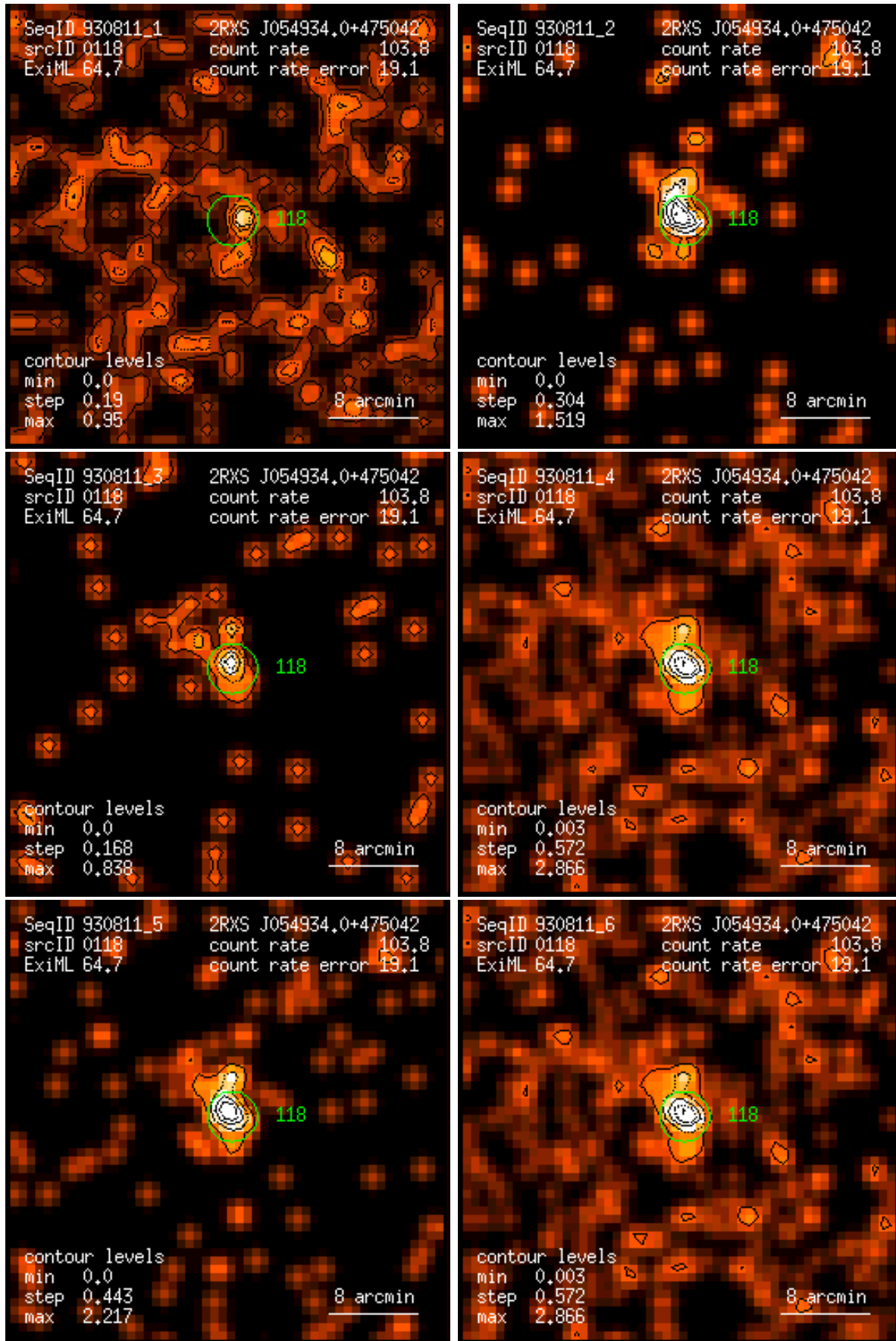
Figure 118: RASS 930811: detection 0118: band rate images, Gaussian filter: (1) PSPC channels 11 – 41, (2) 52 – 90, (3) 91 – 201, (4) 11 – 235, (5) 52 – 201, (6) 11 – 201. Broad band rates in counts/ks. Band rate contour levels in counts/ks/arcmin 2 .
