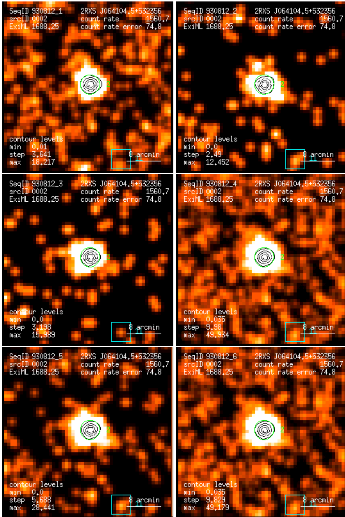
Figure 2: RASS 930812: detection 0002: band rate images, Gaussian filter: (1) PSPC channels 11 – 41, (2) 52 – 90, (3) 91 – 201, (4) 11 – 235, (5) 52 – 201, (6) 11 – 201. Broad band rates in counts/ks. Band rate contour levels in counts/ks/arcmin 2 .
