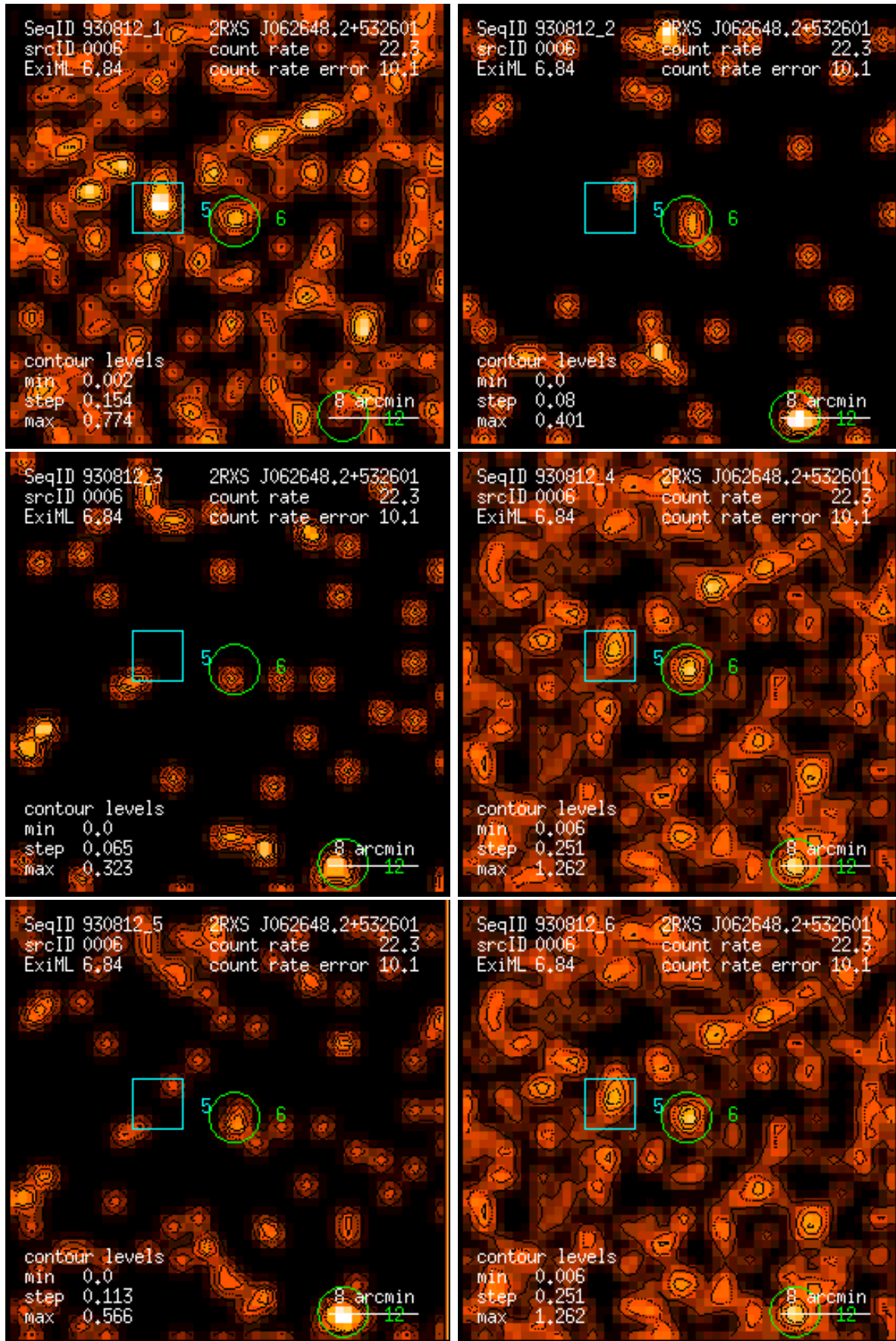
Figure 6: RASS 930812: detection 0006: band rate images, Gaussian filter: (1) PSPC channels 11 – 41, (2) 52 – 90, (3) 91 – 201, (4) 11 – 235, (5) 52 – 201, (6) 11 – 201. Broad band rates in counts/ks. Band rate contour levels in counts/ks/arcmin 2 .
