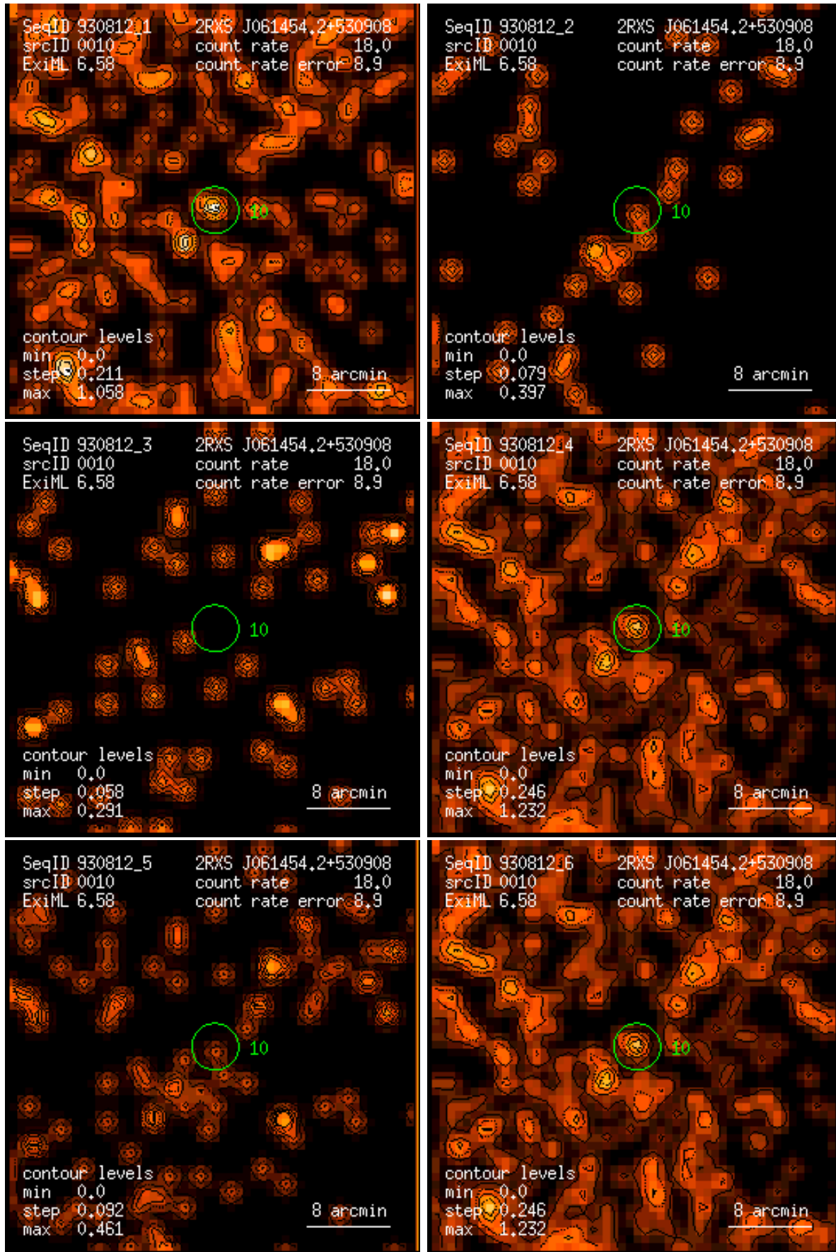
Figure 10: RASS 930812: detection 0010: band rate images, Gaussian filter: (1) PSPC channels 11 – 41, (2) 52 – 90, (3) 91 – 201, (4) 11 – 235, (5) 52 – 201, (6) 11 – 201. Broad band rates in counts/ks. Band rate contour levels in counts/ks/arcmin 2 .
