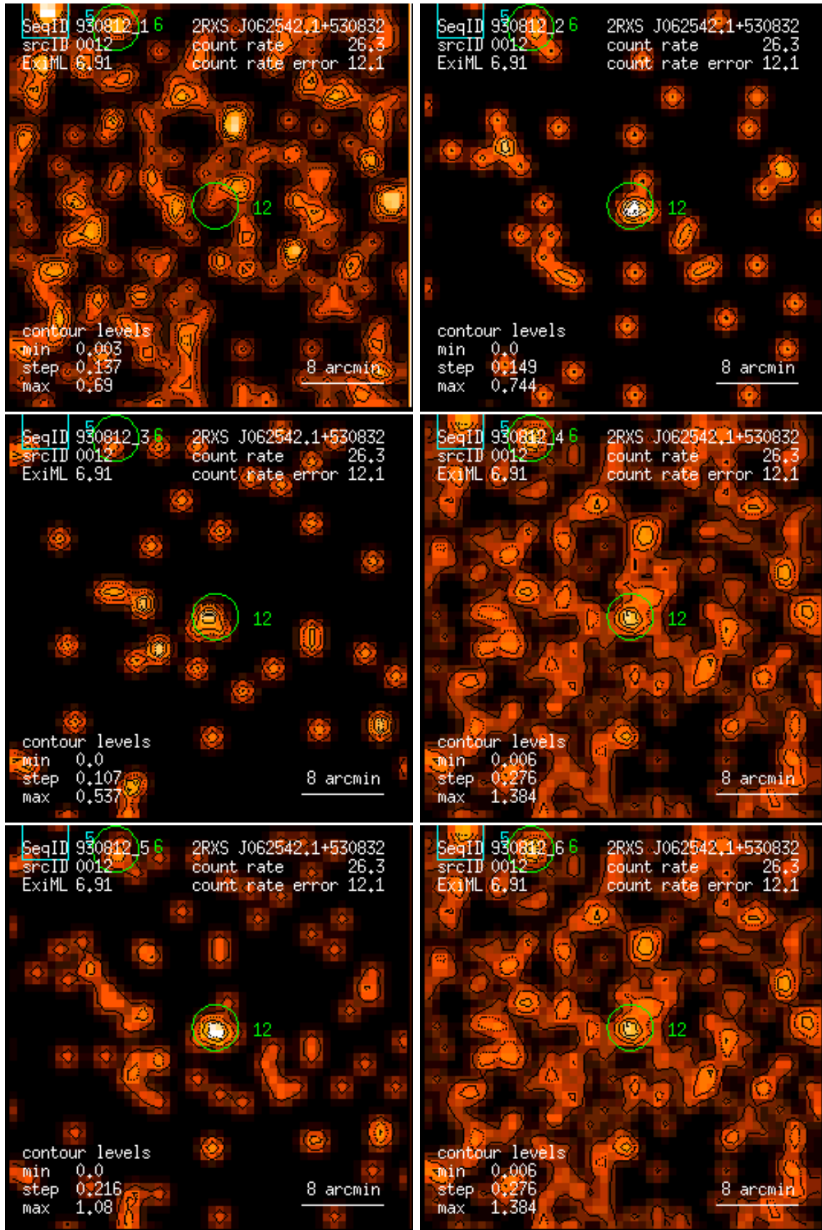
Figure 12: RASS 930812: detection 0012: band rate images, Gaussian filter: (1) PSPC channels 11 – 41, (2) 52 – 90, (3) 91 – 201, (4) 11 – 235, (5) 52 – 201, (6) 11 – 201. Broad band rates in counts/ks. Band rate contour levels in counts/ks/arcmin 2 .
