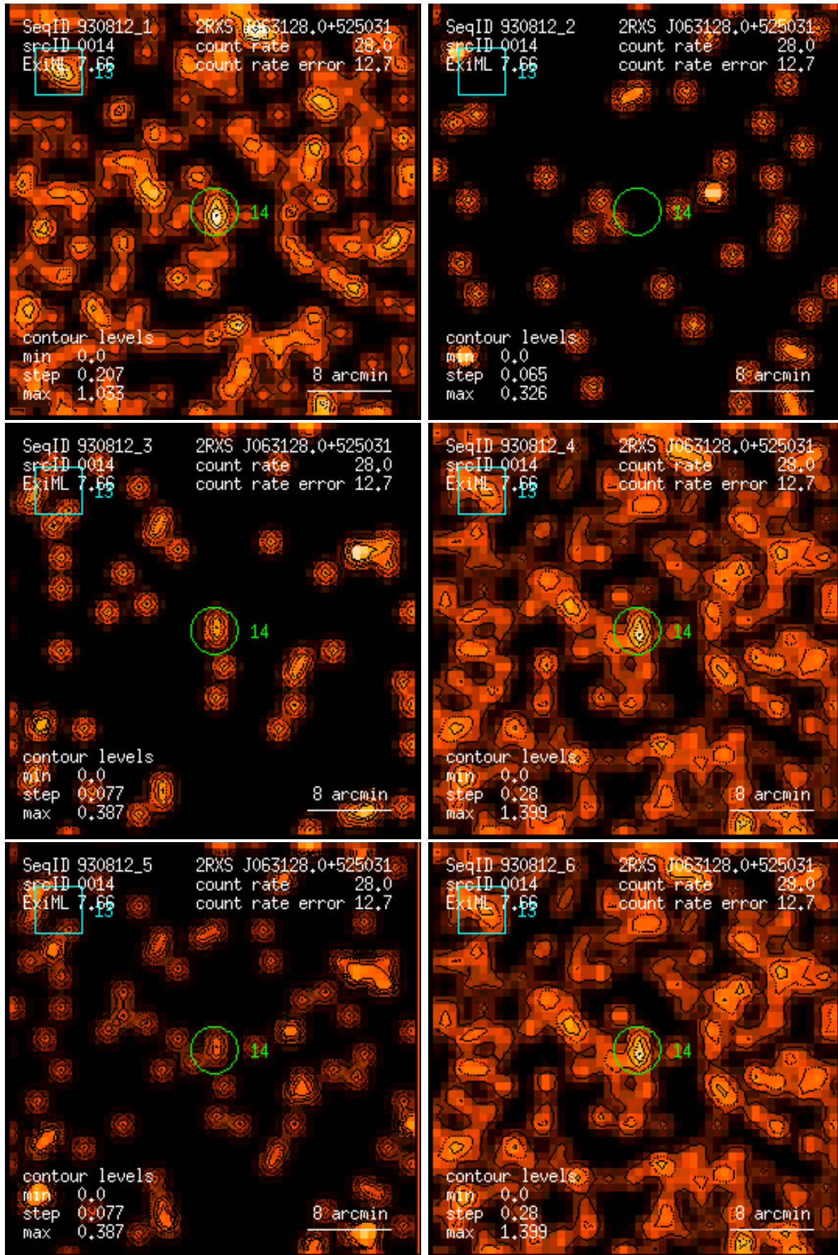
Figure 14: RASS 930812: detection 0014: band rate images, Gaussian filter: (1) PSPC channels 11 – 41, (2) 52 – 90, (3) 91 – 201, (4) 11 – 235, (5) 52 – 201, (6) 11 – 201. Broad band rates in counts/ks. Band rate contour levels in counts/ks/arcmin 2 .
