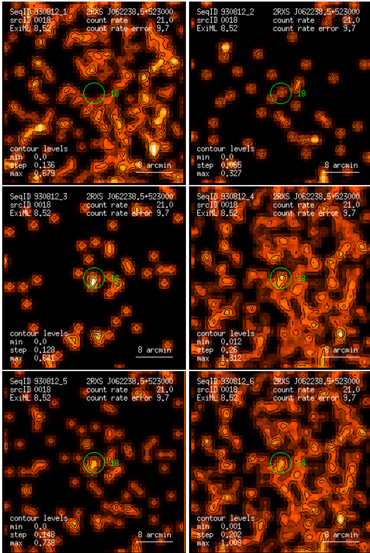
Figure 18: RASS 930812: detection 0018: band rate images, Gaussian filter: (1) PSPC channels 11 – 41, (2) 52 – 90, (3) 91 – 201, (4) 11 – 235, (5) 52 – 201, (6) 11 – 201. Broad band rates in counts/ks. Band rate contour levels in counts/ks/arcmin 2 .
