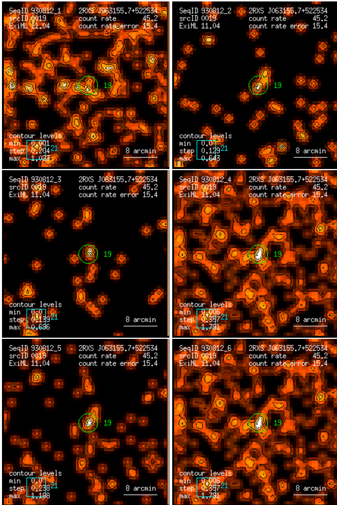
Figure 19: RASS 930812: detection 0019: band rate images, Gaussian filter: (1) PSPC channels 11 – 41, (2) 52 – 90, (3) 91 – 201, (4) 11 – 235, (5) 52 – 201, (6) 11 – 201. Broad band rates in counts/ks. Band rate contour levels in counts/ks/arcmin 2 .
