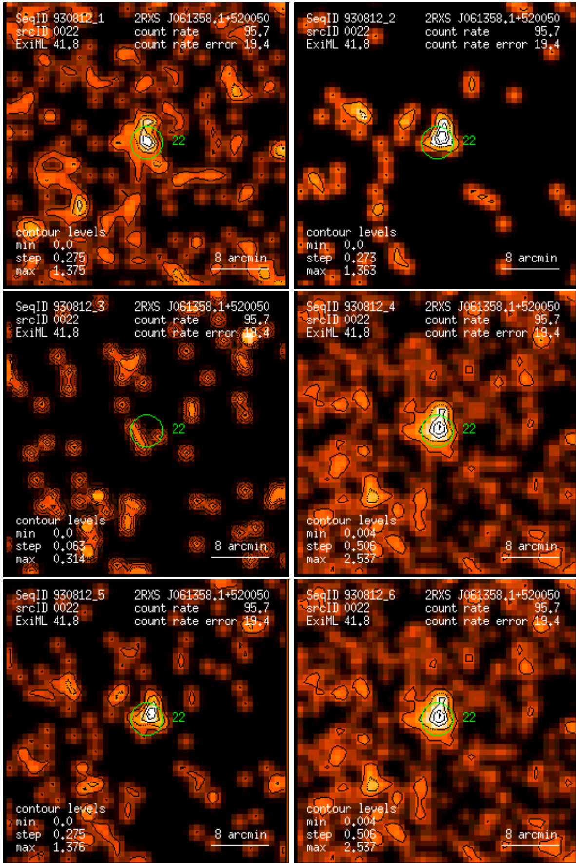
Figure 22: RASS 930812: detection 0022: band rate images, Gaussian filter: (1) PSPC channels 11 – 41, (2) 52 – 90, (3) 91 – 201, (4) 11 – 235, (5) 52 – 201, (6) 11 – 201. Broad band rates in counts/ks. Band rate contour levels in counts/ks/arcmin 2 .
