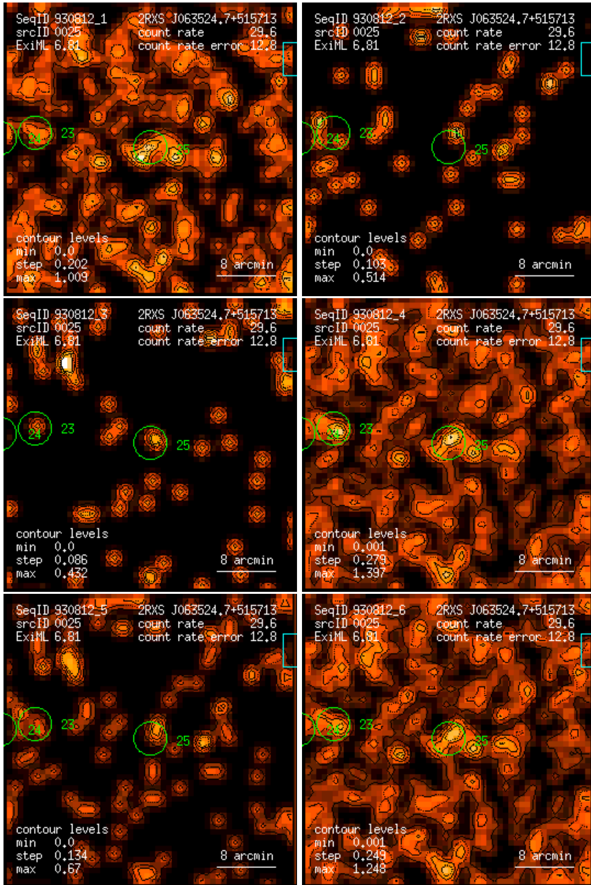
Figure 25: RASS 930812: detection 0025: band rate images, Gaussian filter: (1) PSPC channels 11 – 41, (2) 52 – 90, (3) 91 – 201, (4) 11 – 235, (5) 52 – 201, (6) 11 – 201. Broad band rates in counts/ks. Band rate contour levels in counts/ks/arcmin 2 .
