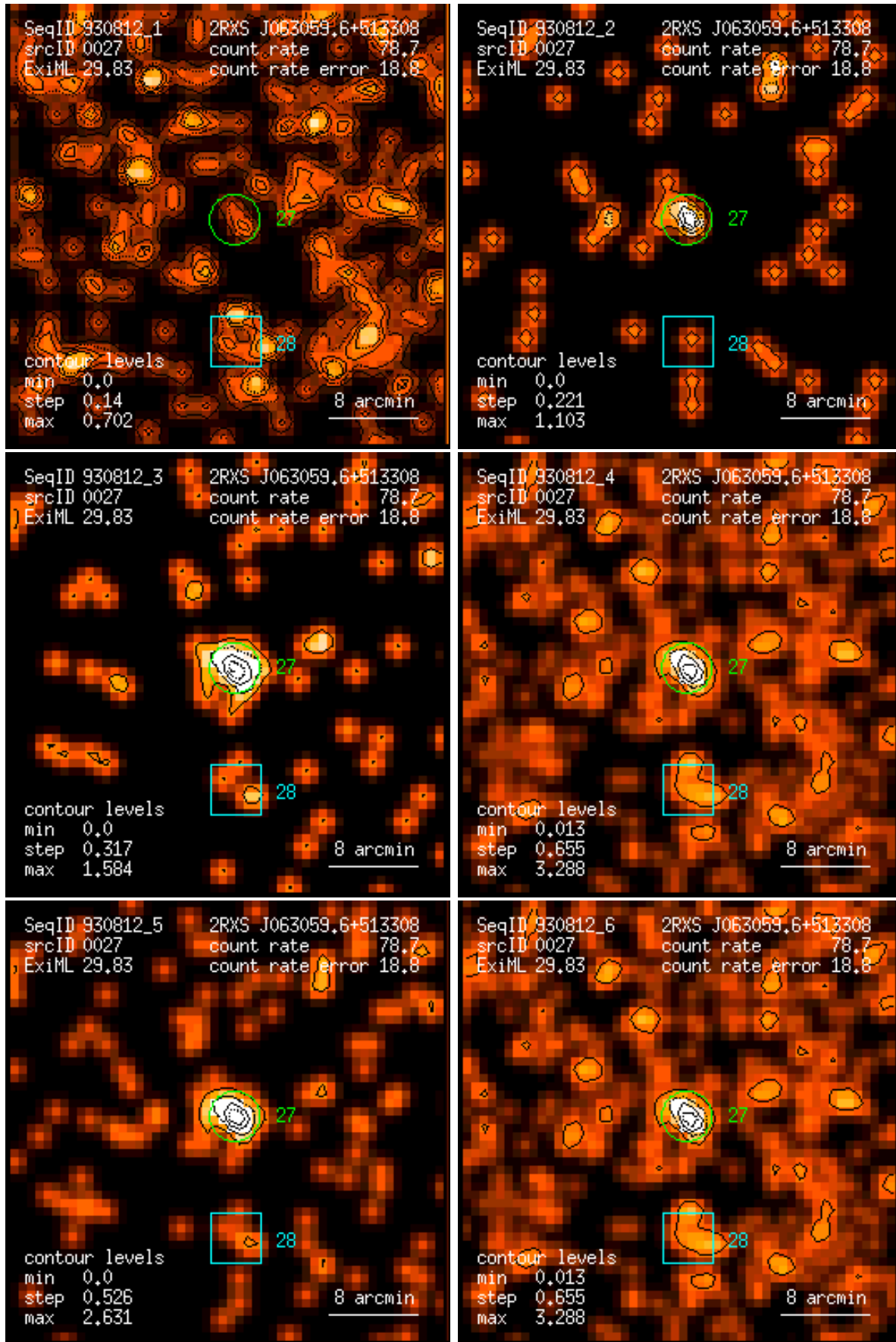
Figure 27: RASS 930812: detection 0027: band rate images, Gaussian filter: (1) PSPC channels 11 – 41, (2) 52 – 90, (3) 91 – 201, (4) 11 – 235, (5) 52 – 201, (6) 11 – 201. Broad band rates in counts/ks. Band rate contour levels in counts/ks/arcmin 2 .
