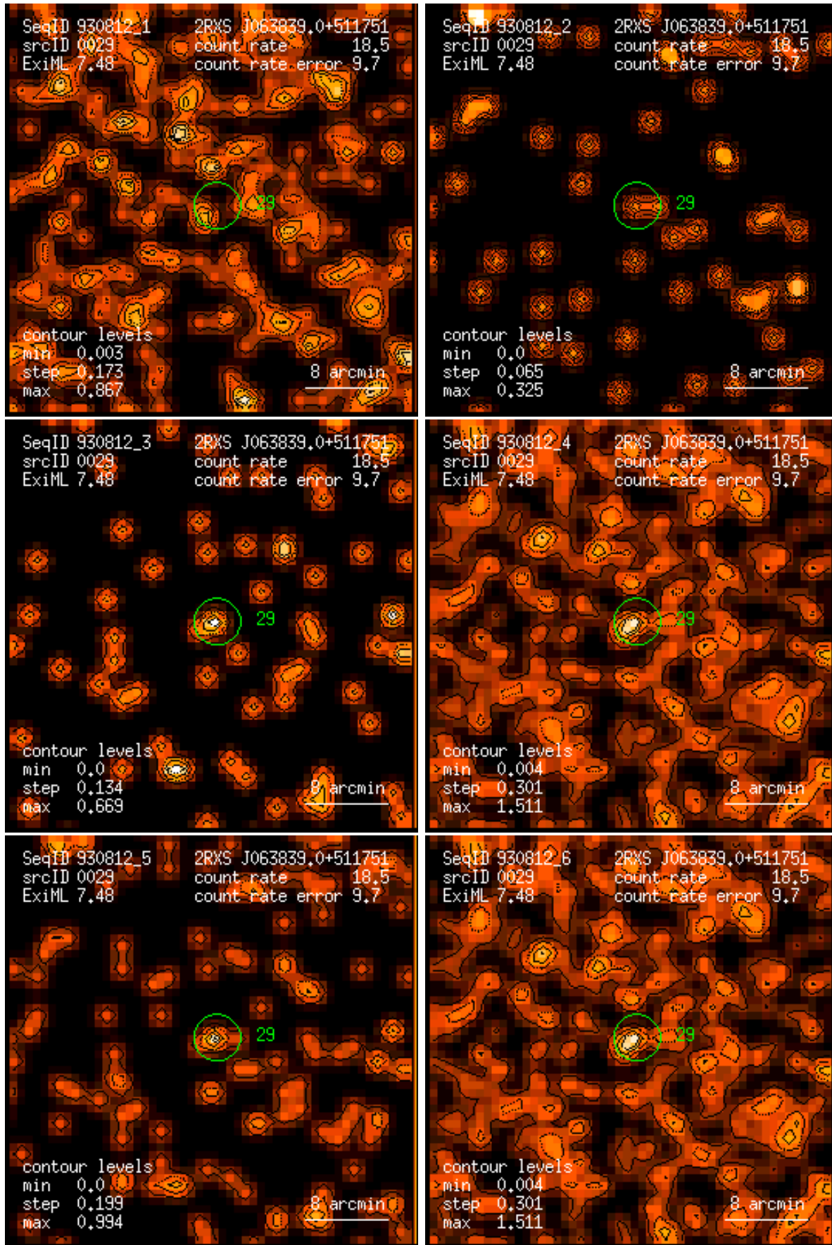
Figure 29: RASS 930812: detection 0029: band rate images, Gaussian filter: (1) PSPC channels 11 – 41, (2) 52 – 90, (3) 91 – 201, (4) 11 – 235, (5) 52 – 201, (6) 11 – 201. Broad band rates in counts/ks. Band rate contour levels in counts/ks/arcmin 2 .
