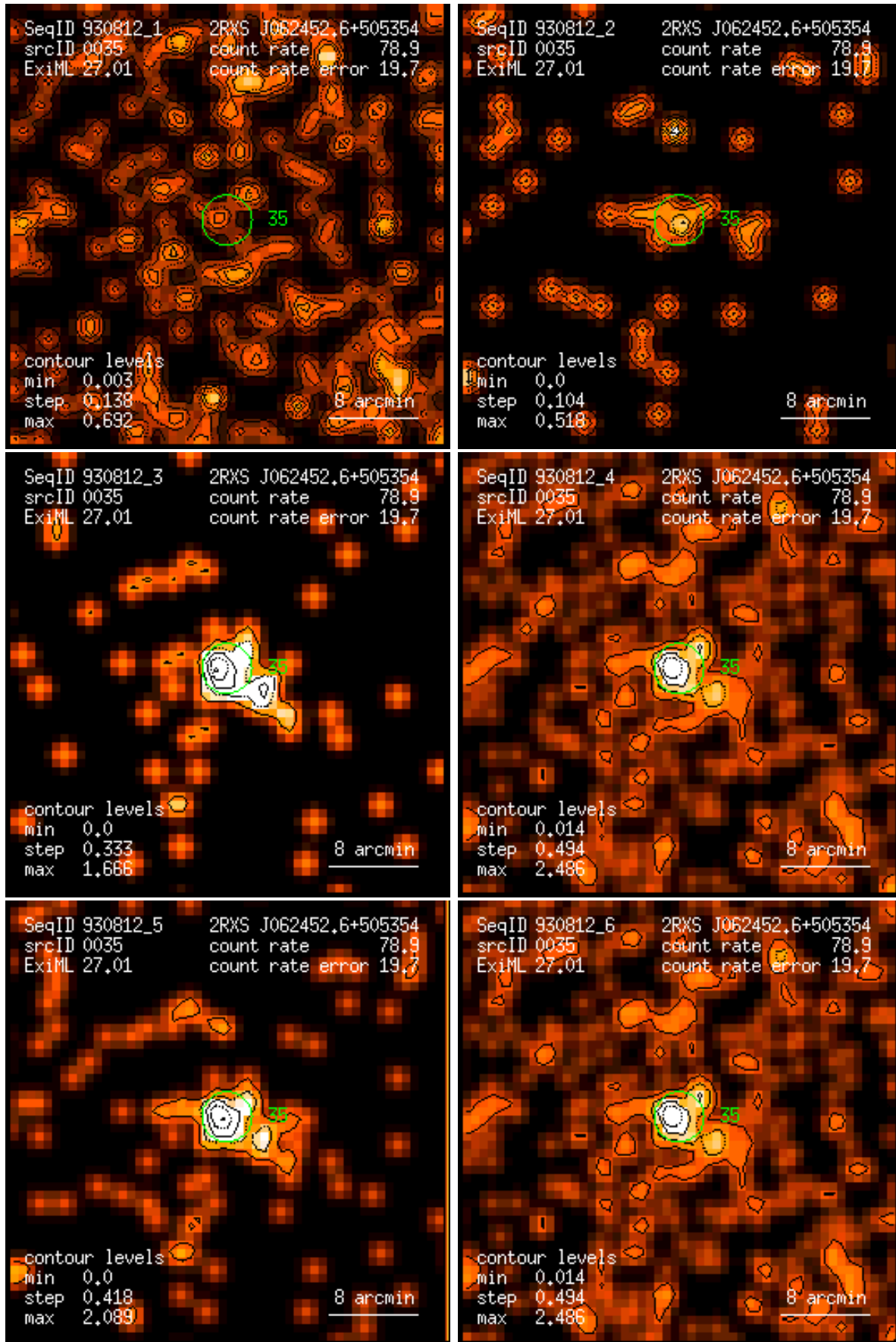
Figure 35: RASS 930812: detection 0035: band rate images, Gaussian filter: (1) PSPC channels 11 – 41, (2) 52 – 90, (3) 91 – 201, (4) 11 – 235, (5) 52 – 201, (6) 11 – 201. Broad band rates in counts/ks. Band rate contour levels in counts/ks/arcmin 2 .
